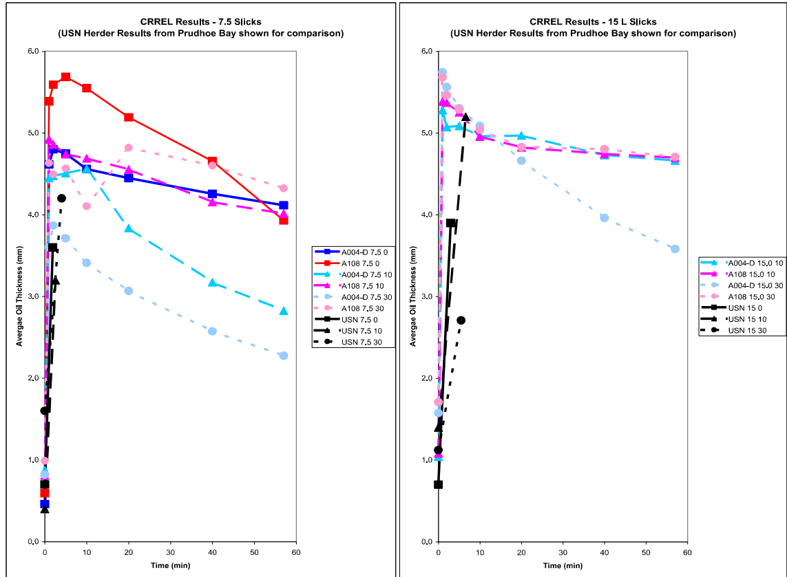
Figure 29. CRREL results with 7.5 L and 15 L slicks
