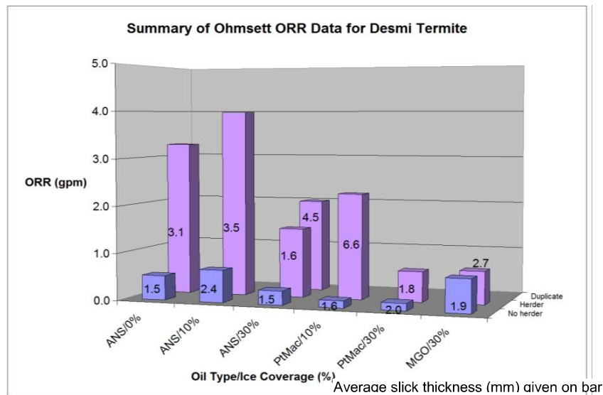
Figure 32. ORR results for weir skimmer experiments.
