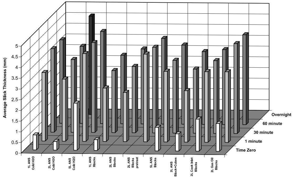
Figure 4. Results of 10-m 2 pan tests.
