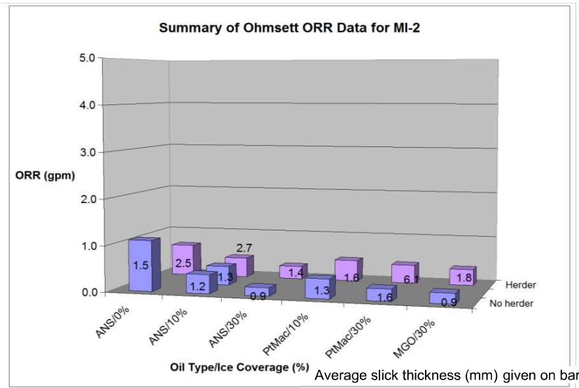
Figure 33. ORR results for oleophilic disc skimmer.
