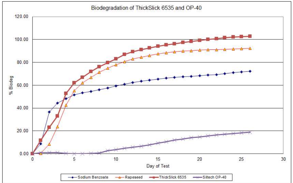
Figure 42. Biodegradation curves for ThickSlick 6535 and Siltech OP-40
