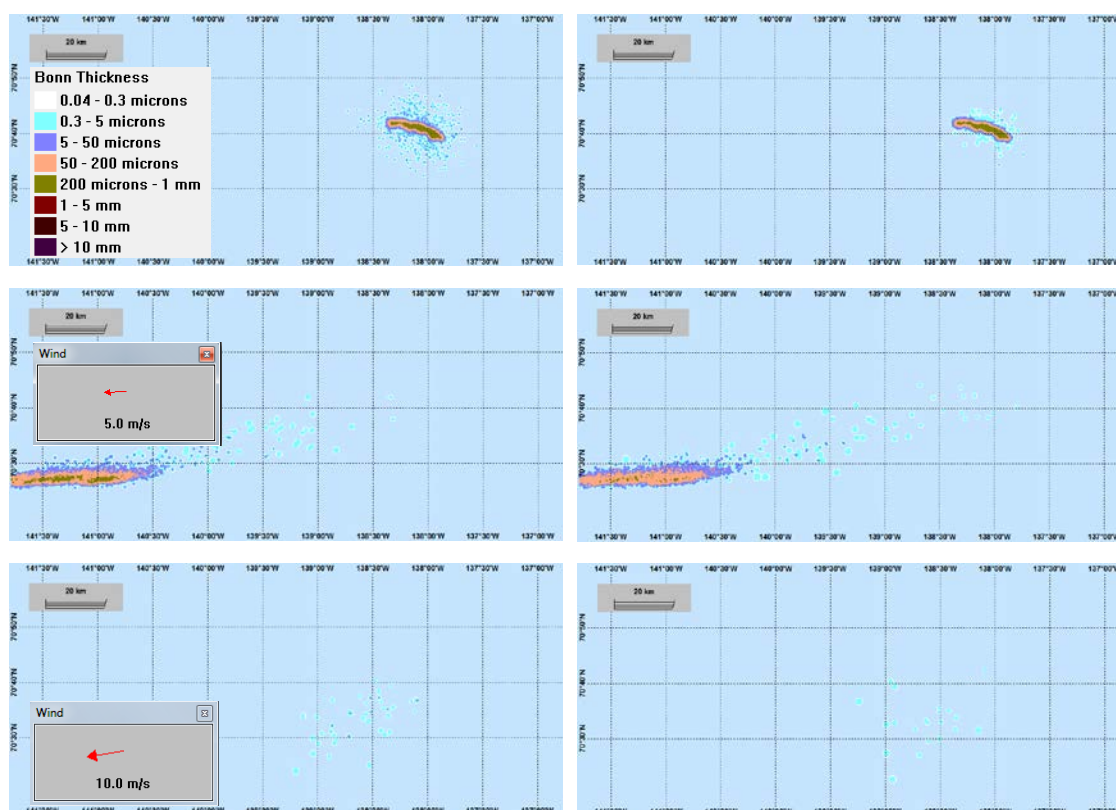
Figure 4.8 Surface oil at the end of the simulation period (10 days) for releases at 150 m depth. Left – oil only: No wind (upper), 5 m/s wind (middle) and 10 m/s wind (lower). Right – with SSDI: No wind (upper), 5 m/s wind (middle) and 10 m/s wind (lower).
