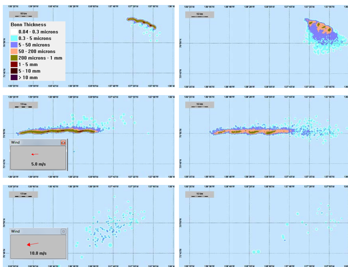
Figure 4.19 Surface oil 5 days into the simulation period (3 days after the end of the release) for releases at 700 m depth. Left – oil only: No wind (upper), 5 m/s wind (middle) and 10 m/s wind (lower). Right – with SSDI: No wind (upper), 5 m/s wind (middle) and 10 m/s wind (lower).
