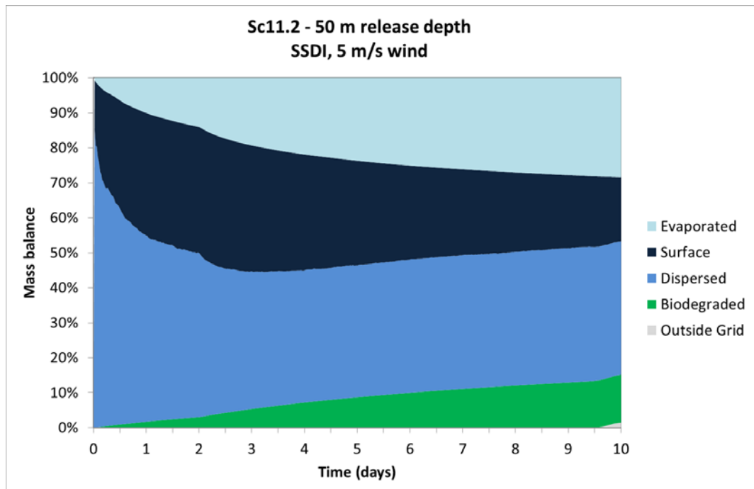
Figure A 8 Mass balance scenario 11.2
