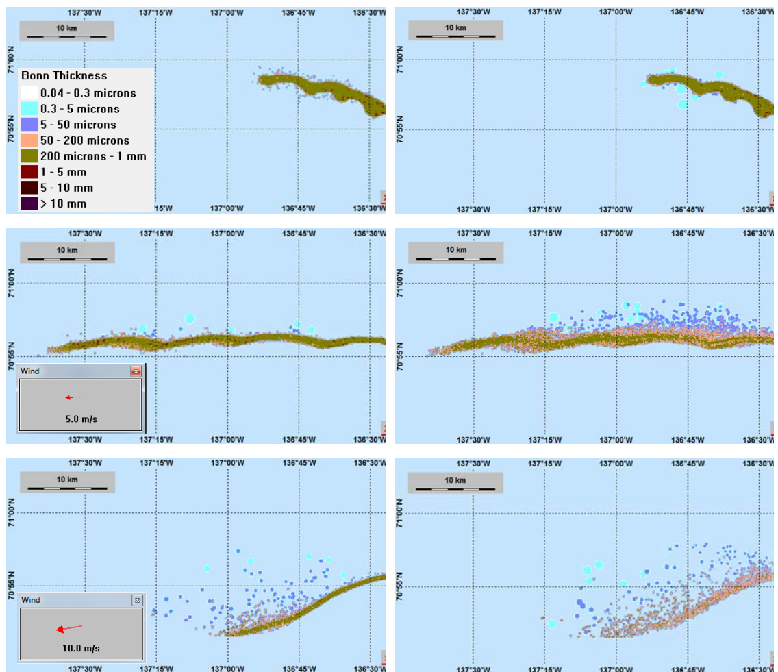
Figure 4.6 Surface oil at the end of the release (2 days) for releases at 150 m depth. Left – oil only: No wind (upper), 5 m/s wind (middle) and 10 m/s wind (lower). Right – with SSDI: No wind (upper), 5 m/s wind (middle) and 10 m/s wind (lower).
