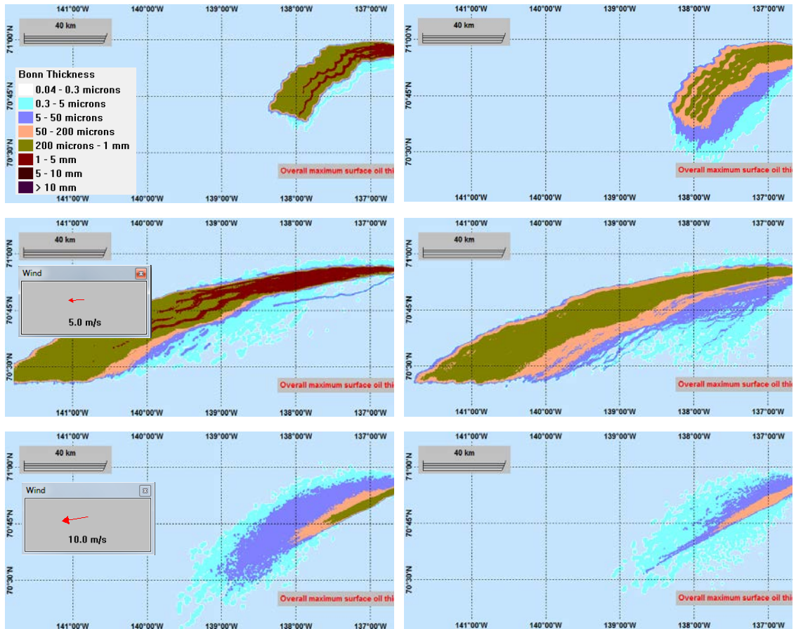
Figure 4.23 Overall maximum surface oil thickness for all releases at 700 m (impacted area. Left – oil only: No wind (upper), 5 m/s wind (middle) and 10 m/s wind (lower). Right – with SSDI: No wind (upper), 5 m/s wind (middle) and 10 m/s wind (lower).
