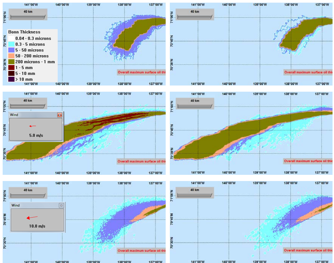
Figure 4.11 Overall maximum surface oil thickness (impacted area) for all scenarios with release at 150 m. Left – oil only: No wind (upper), 5 m/s wind (middle) and 10 m/s wind (lower). Right – with SSDI: No wind (upper), 5 m/s wind (middle) and 10 m/s wind (lower).
