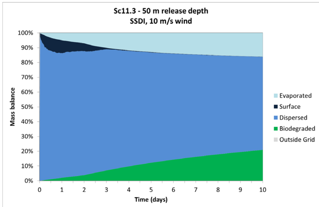
Figure A 9 Mass balance scenario 11.3
