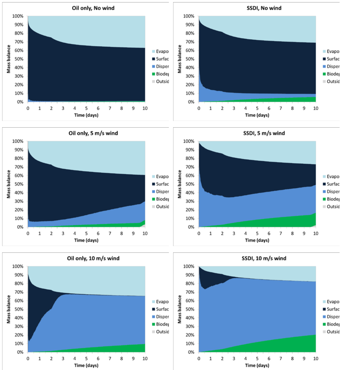
Figure 4.9 Mass balance for all scenarios with releases at 150 m depth. Left – oil only: No wind (upper), 5 m/s wind (middle) and 10 m/s wind (lower). Right – with SSDI: No wind (upper), 5 m/s wind (middle) and 10 m/s wind (lower).
