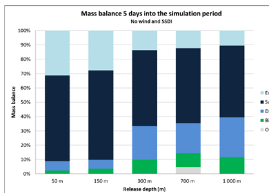
Figure 2.3 Example of mass balance comparison between several simulations without wind and with subsea injection, where the mass balance is obtained 5 days into the simulation period. The legend "outside" represents the oil that is outside the geographical grid defined for the modelling.
