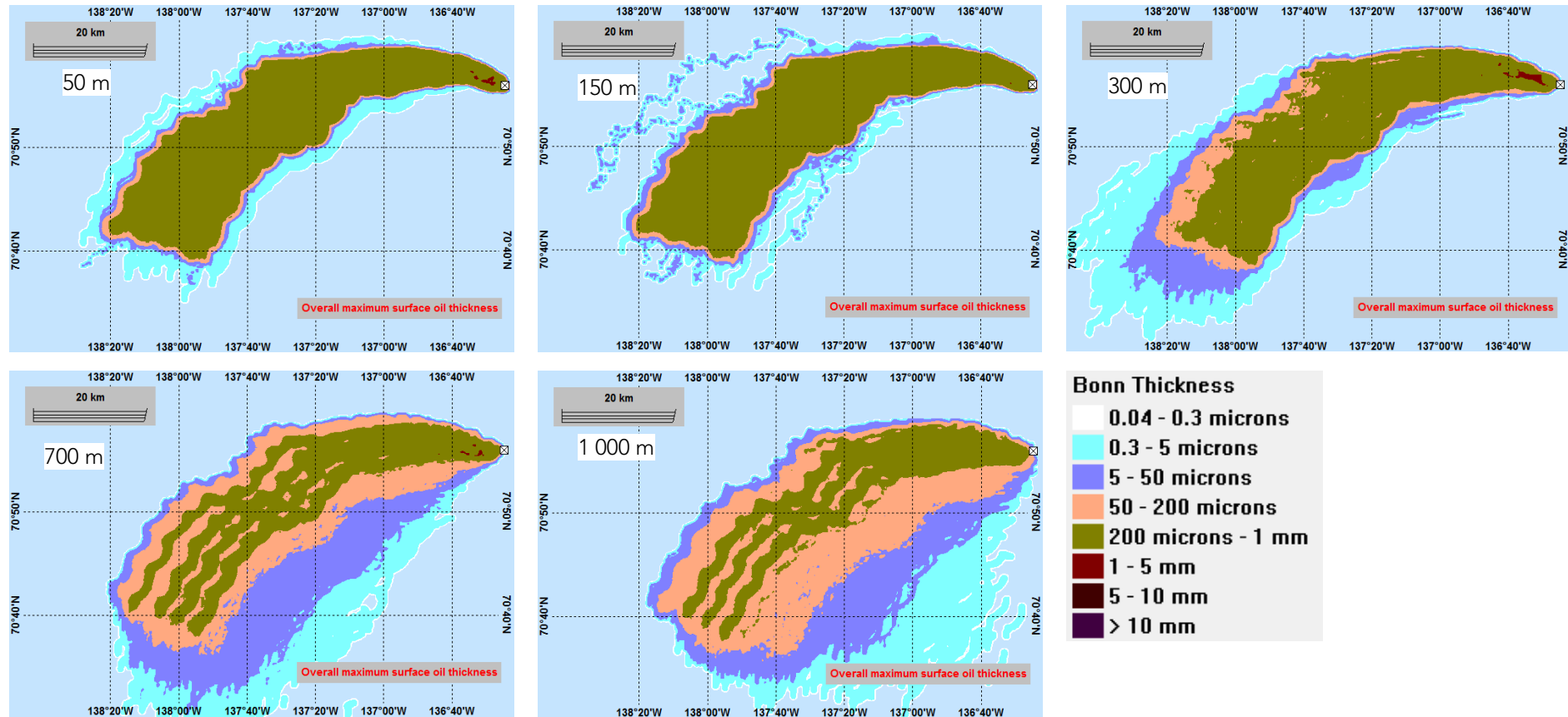
Figure 4.5 Overall maximum surface oil thickness (impacted surface area) for all release depths (scenarios 11.1-15.1), without wind and with SSDI.
