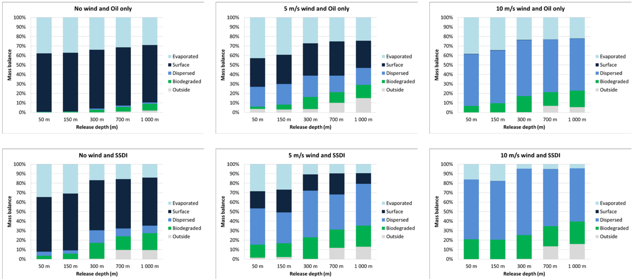
Figure 4.3 Mass balance at the end of the simulation period (10 days) for all scenarios. The upper pictures show the results for the scenarios without SSDI, whereas the lower pictures are the scenarios with SSDI. Left: No wind. Middle: 5 m/s wind. Right: 10 m/s wind.
