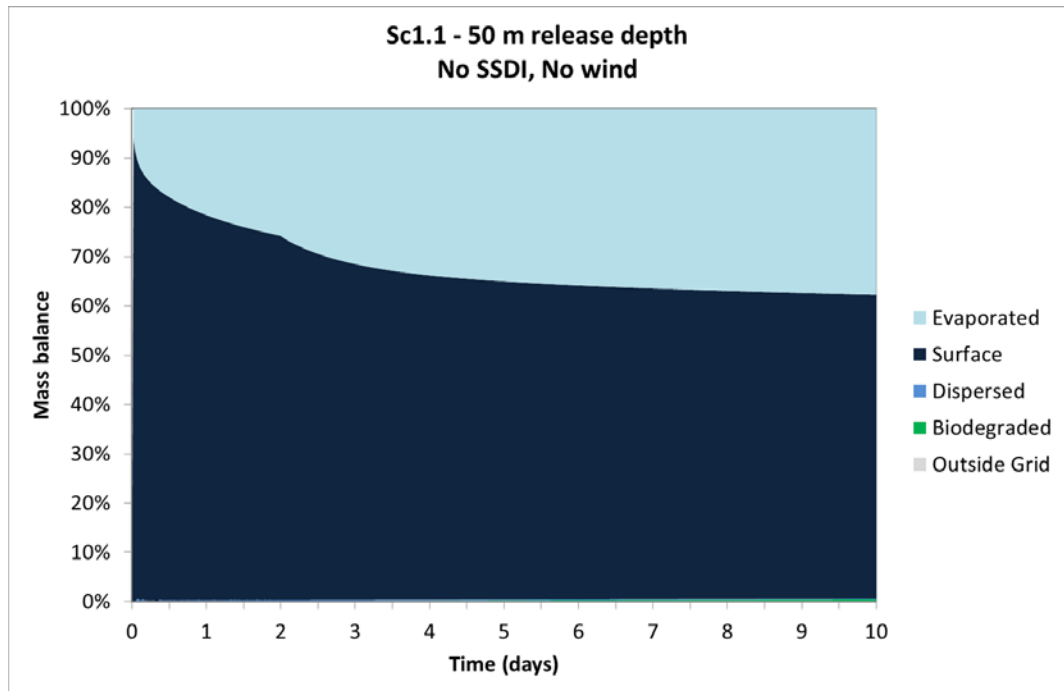
Figure A 1 Mass balance scenario 1.1
