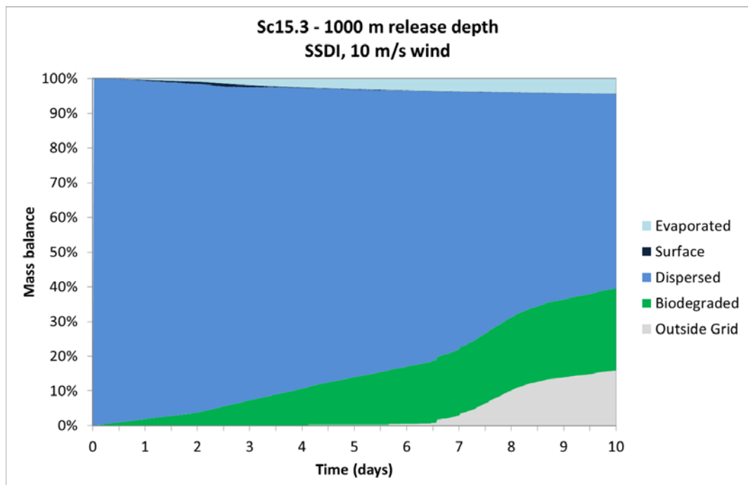
Figure A 12 Mass balance scenario 15.3
