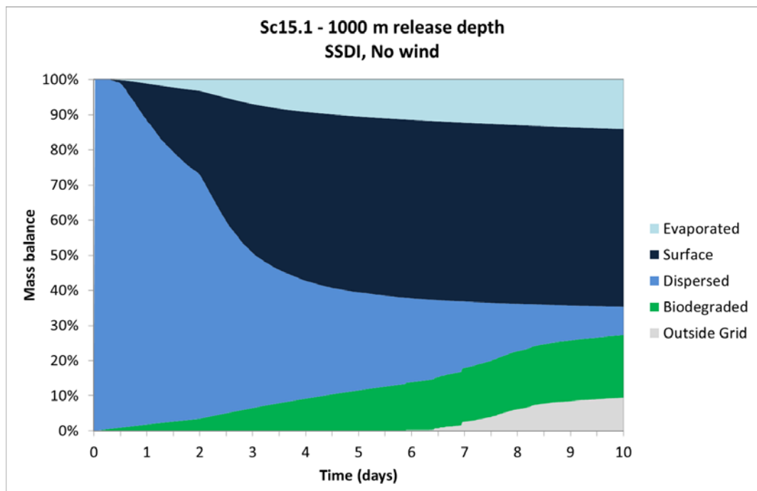
Figure A 10 Mass balance scenario 15.1
