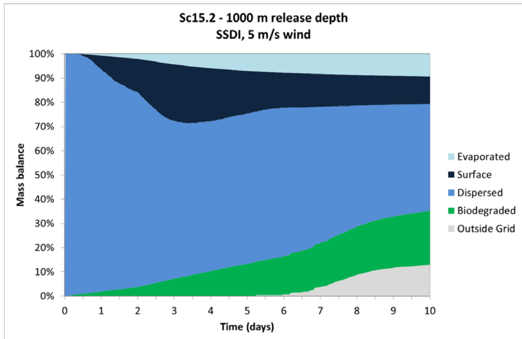
Figure A 11 Mass balance scenario 15.2
