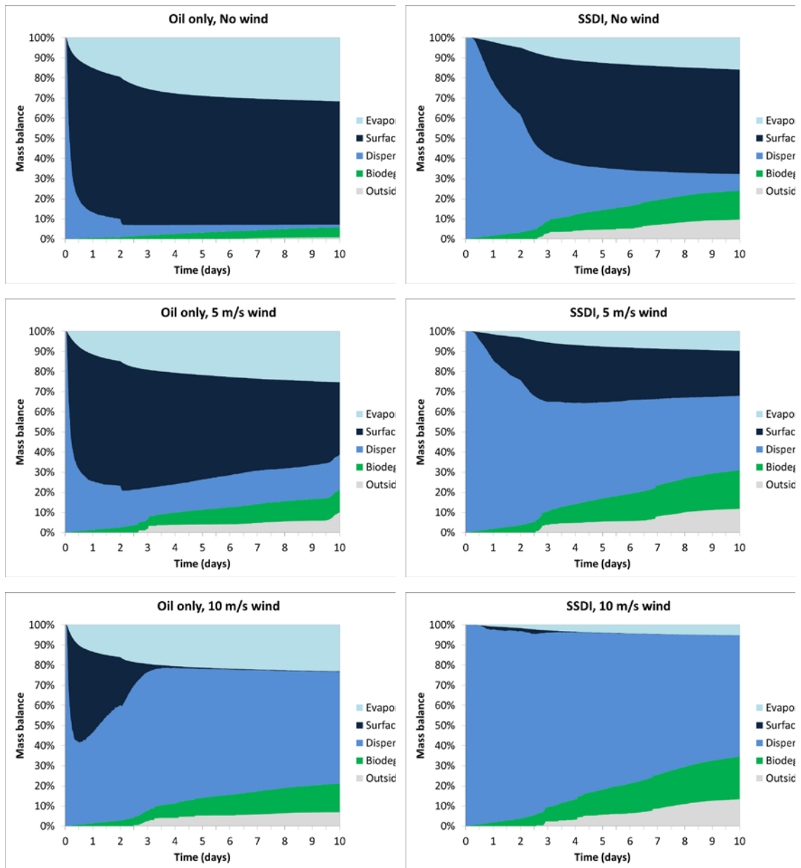
Figure 4.21 Mass balance for all scenarios with releases at 700 m depth. Left – oil only: No wind (upper), 5 m/s wind (middle) and 10 m/s wind (lower). Right – with SSDI: No wind (upper), 5 m/s wind (middle) and 10 m/s wind (lower).
