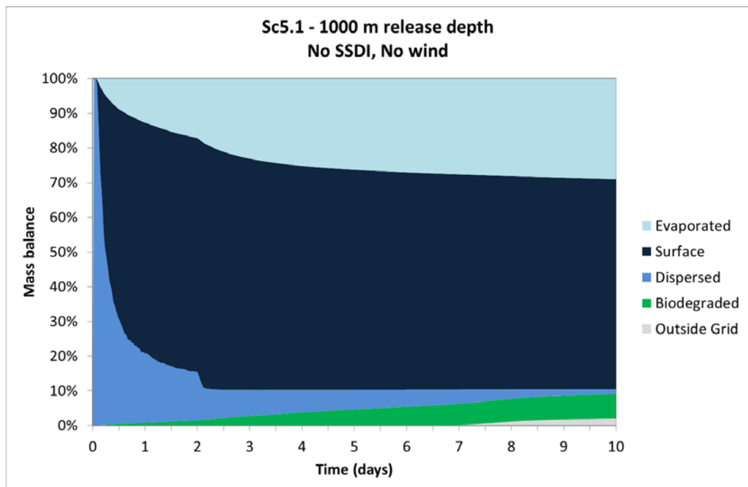
Figure A 4 Mass balance scenario 5.1
