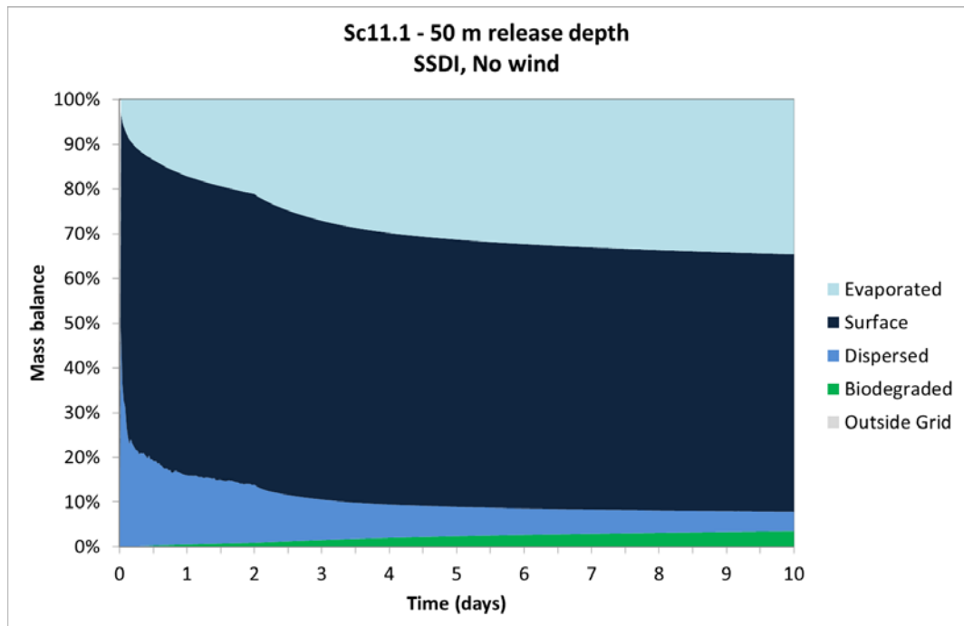
Figure A 7 Mass balance scenario 11.1
