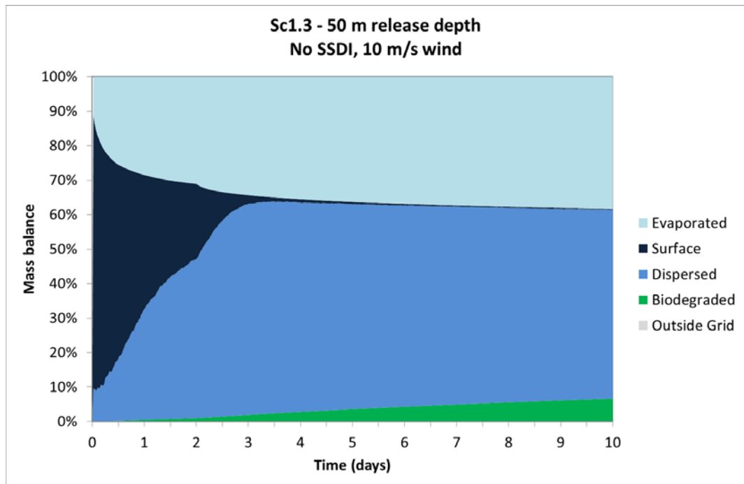
Figure A 3 Mass balance scenario 1.3
