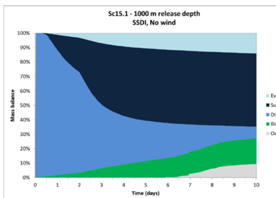
Figure 2.2 Example of mass balance for a simulation without wind and with subsea dispersant injection as a function of time, from start of release to end of release (day 2) and continued to the end of simulation (day 10).
