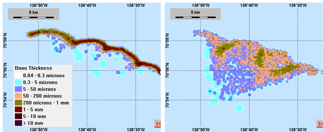
Figure 5.4 Surface oil at the end of the release (2 days into the simulation period) for the scenarios with release depth 700 m and without wind. Left: Oil only. Right: SSDI applied.
