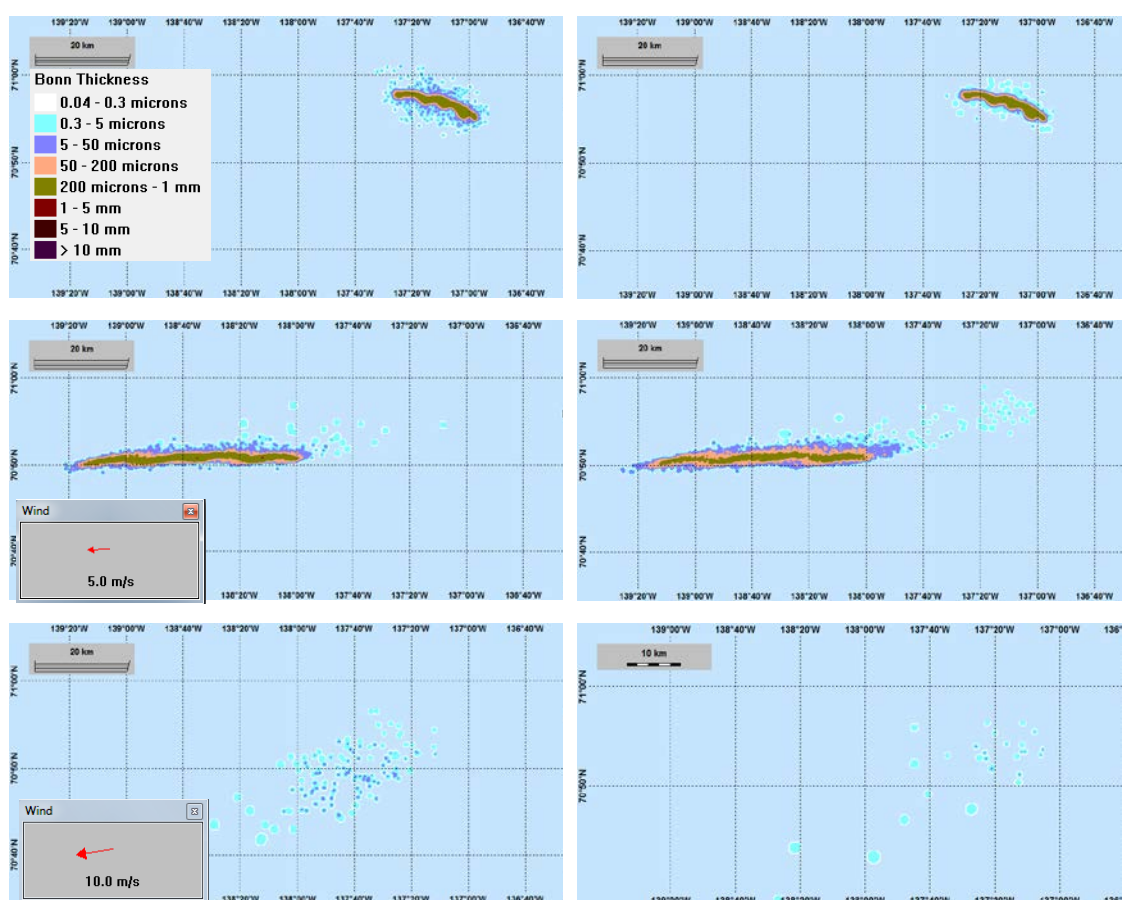
Figure 4.7 Surface oil 5 days into the simulation period (3 days after the end of the release) for releases at 150 m depth. Left – oil only: No wind (upper), 5 m/s wind (middle) and 10 m/s wind (lower). Right – with SSDI: No wind (upper), 5 m/s wind (middle) and 10 m/s wind (lower).
