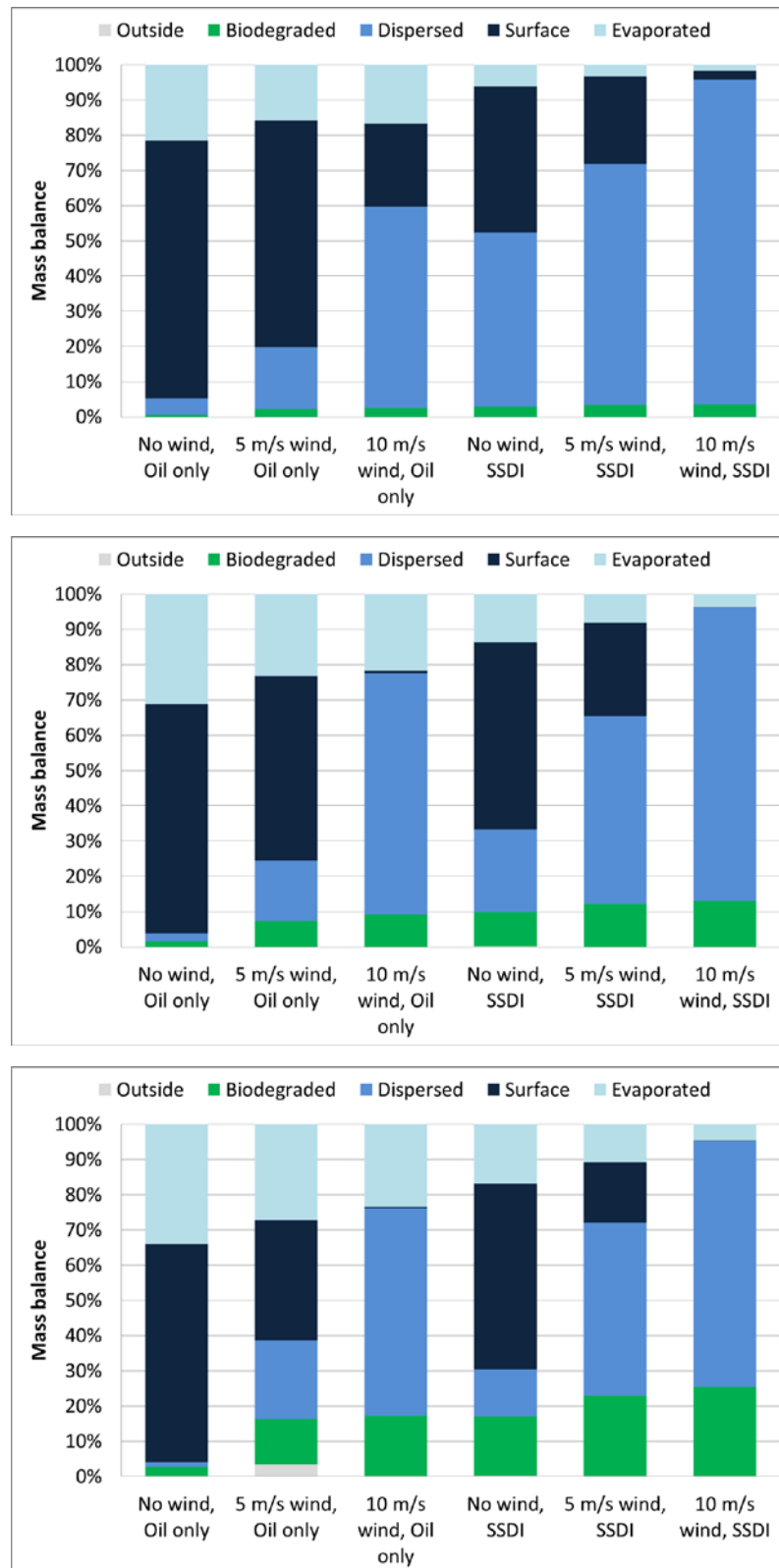
Figure 4.16 Mass balance at the end of the release (2 days into the simulation) (upper), 5 days (middle) and 10 days (lower) into the simulation period at 300 m depth with and without the presence of wind and SSDI.
