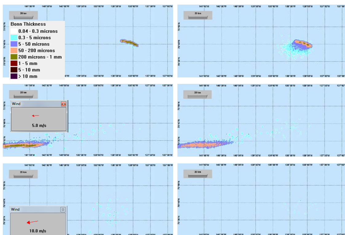
Figure 4.14 Surface oil at the end of the simulation period (10 days) for releases at 300 m depth. Left – oil only: No wind (upper), 5 m/s wind (middle) and 10 m/s wind (lower). Right – with SSDI: No wind (upper), 5 m/s wind (middle) and 10 m/s wind (lower).
