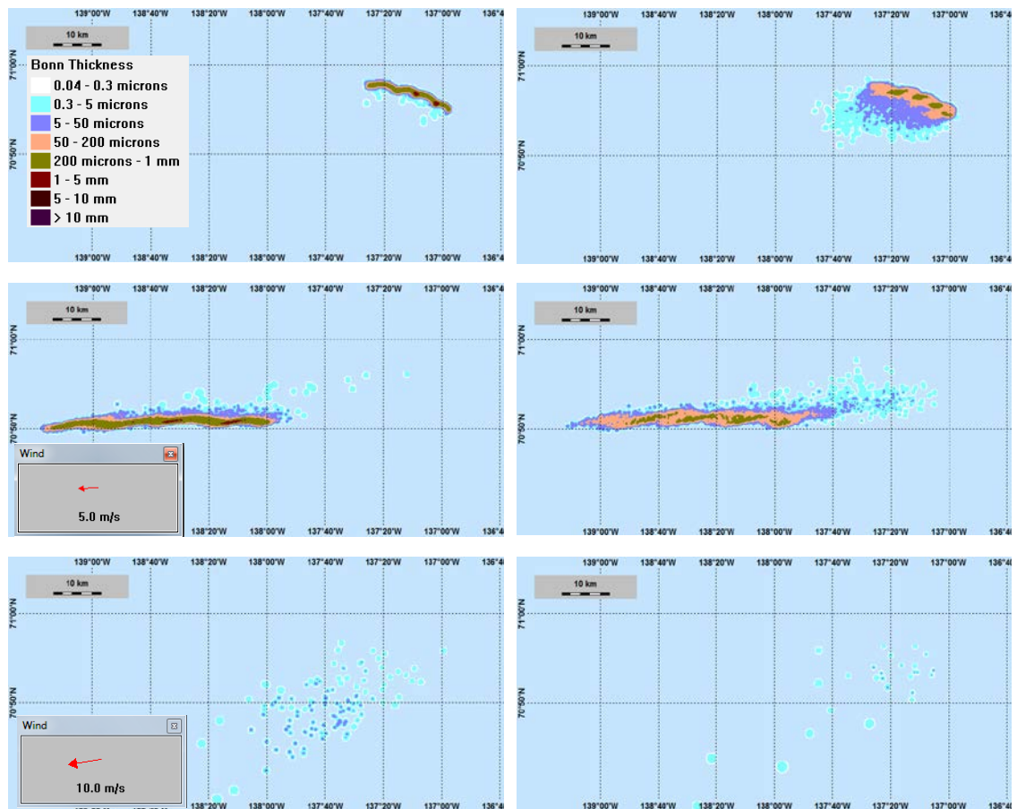
Figure 4.13 Surface oil 5 days into the simulation period (3 days after the end of the release) for releases at 300 m depth. Left – oil only: No wind (upper), 5 m/s wind (middle) and 10 m/s wind (lower). Right – with SSDI: No wind (upper), 5 m/s wind (middle) and 10 m/s wind (lower).
