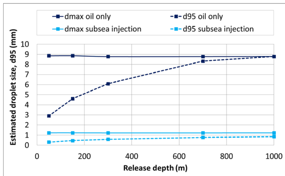
Figure 5.1 Estimated d_{95} and d_{max} at the different release depths for the scenarios with and without subsea injection of dispersants.
