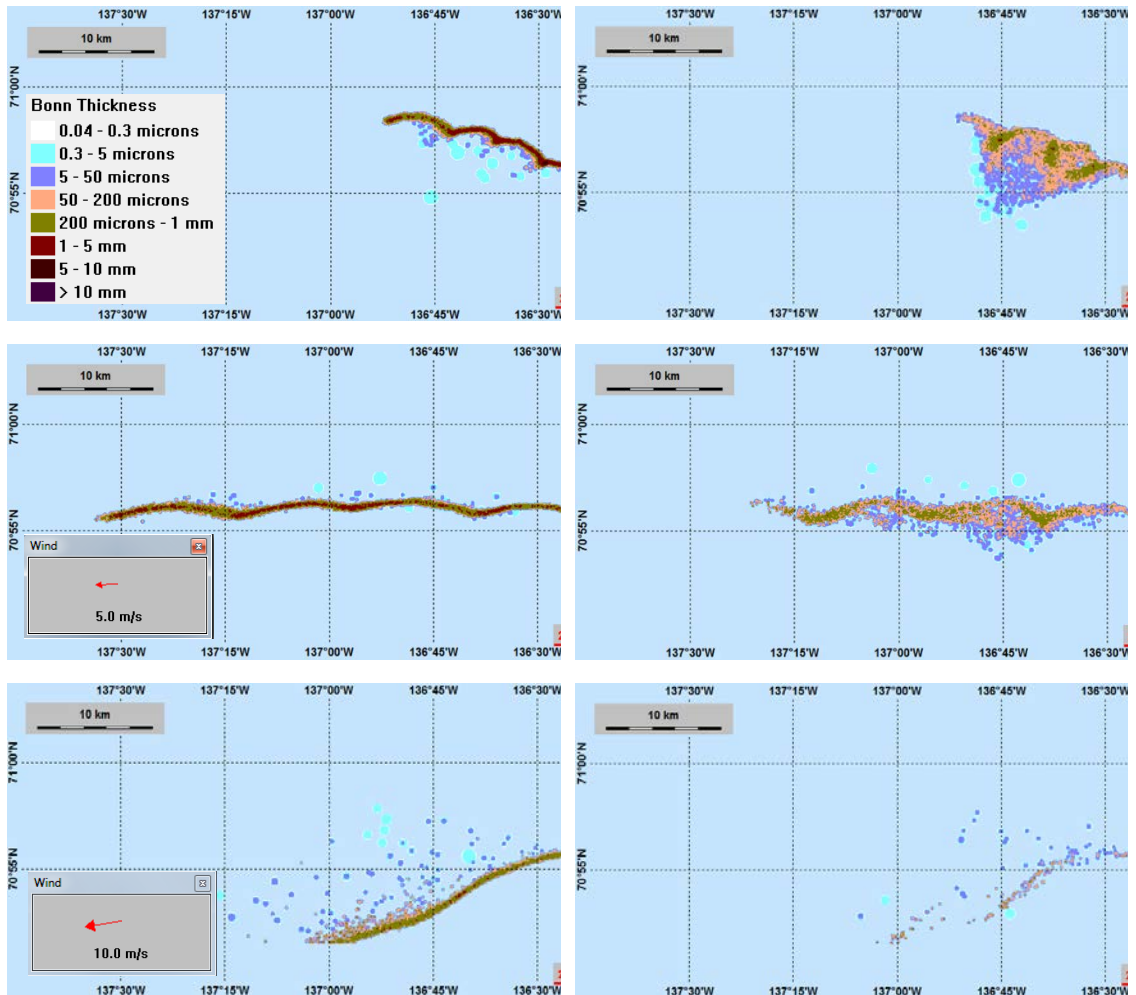
Figure 4.18 Surface oil at the end of the release for releases at 700 m depth. Left – oil only: No wind (upper), 5 m/s wind (middle) and 10 m/s wind (lower). Right – with SSDI: No wind (upper), 5 m/s wind (middle) and 10 m/s wind (lower).
