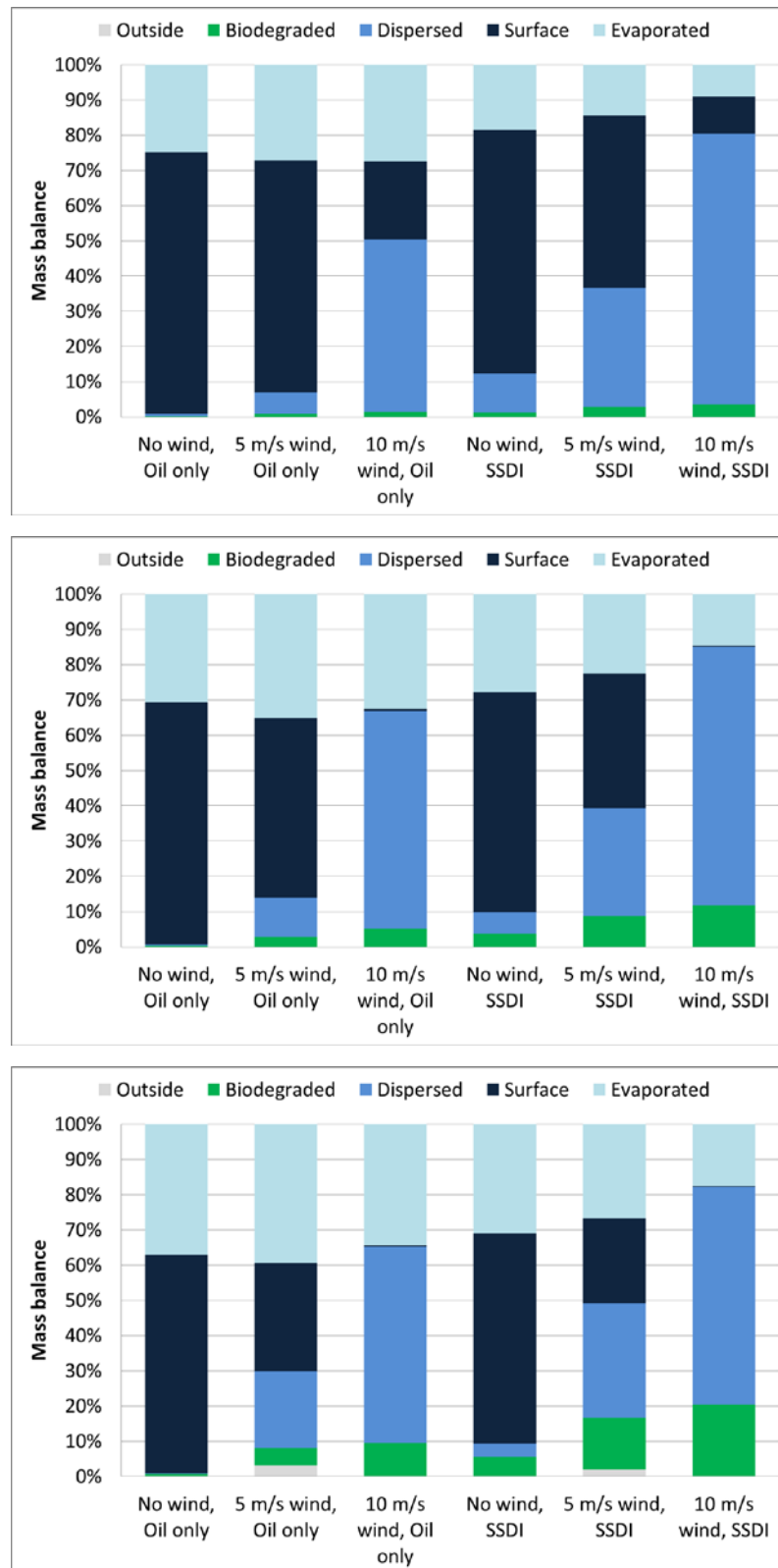
Figure 4.10 Mass balance at the end of the release (2 days into the simulation) (upper), 5 days (middle) and 10 days (lower) into the simulation period at 150 m depth with and without the presence of wind and SSDI.
