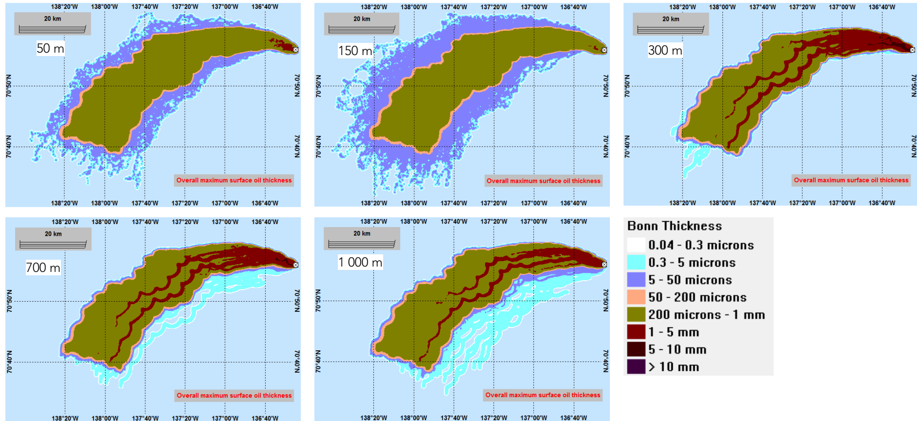
Figure 4.4 Overall maximum surface oil thickness (impacted surface area) for all release depths (scenarios 1.1-5.1), without wind and with oil only.
