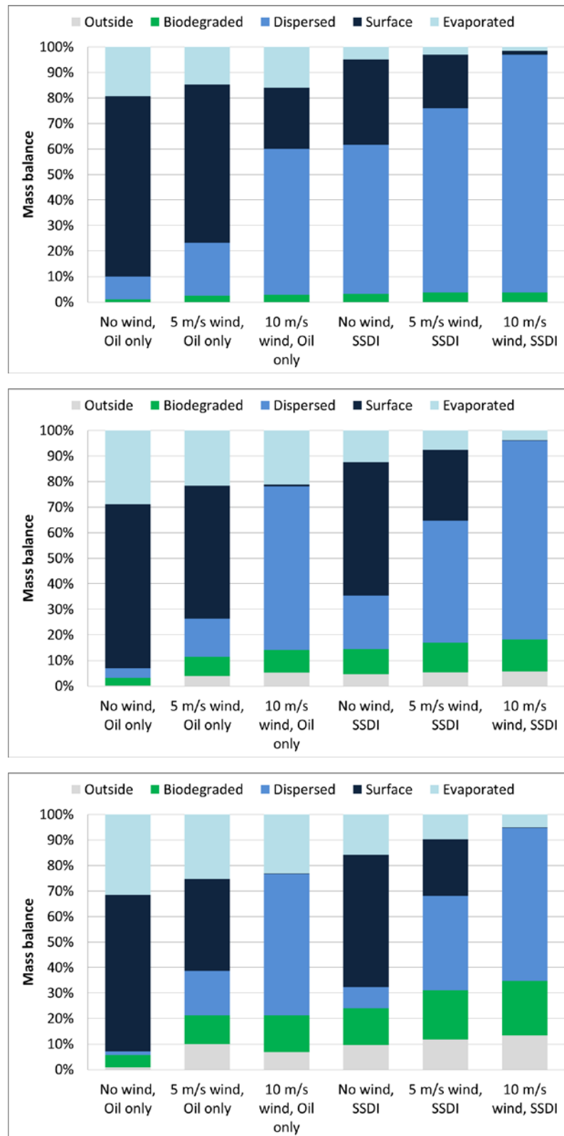
Figure 4.22 Mass balance at the end of the release (2 days into the simulation) (upper), 5 days (middle) and 10 days (lower) into the simulation period at 700 m depth with and without the presence of wind and SSDI.
