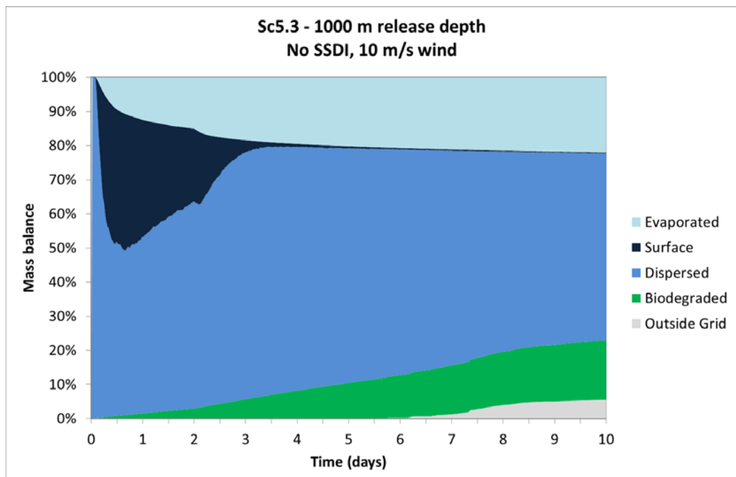
Figure A 6 Mass balance scenario 5.3
