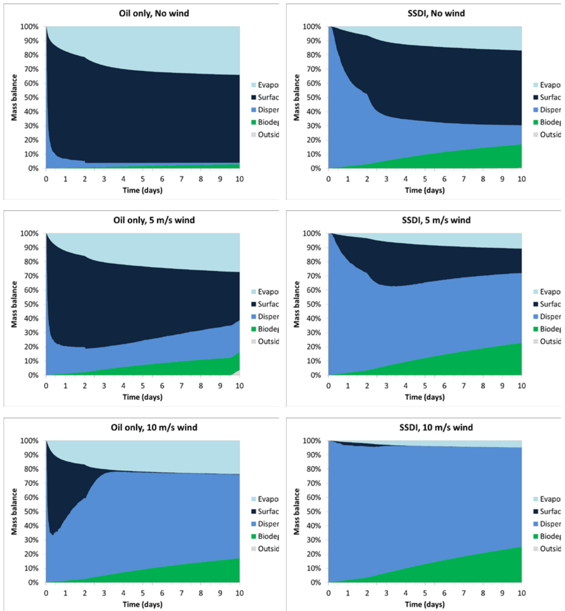
Figure 4.15 Mass balance for all scenarios with releases at 300 m depth. Left – oil only: No wind (upper), 5 m/s wind (middle) and 10 m/s wind (lower). Right – with SSDI: No wind (upper), 5 m/s wind (middle) and 10 m/s wind (lower).
