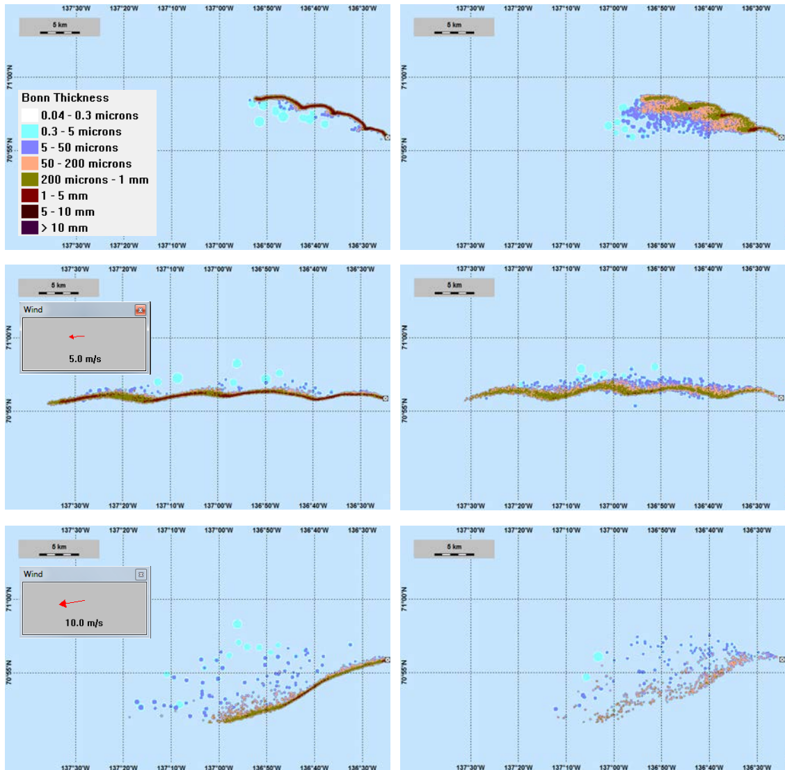
Figure 4.12 Surface oil at the end of the release for releases at 300 m depth. Left – oil only: No wind (upper), 5 m/s wind (middle) and 10 m/s wind (lower). Right – with SSDI: No wind (upper), 5 m/s wind (middle) and 10 m/s wind (lower).
