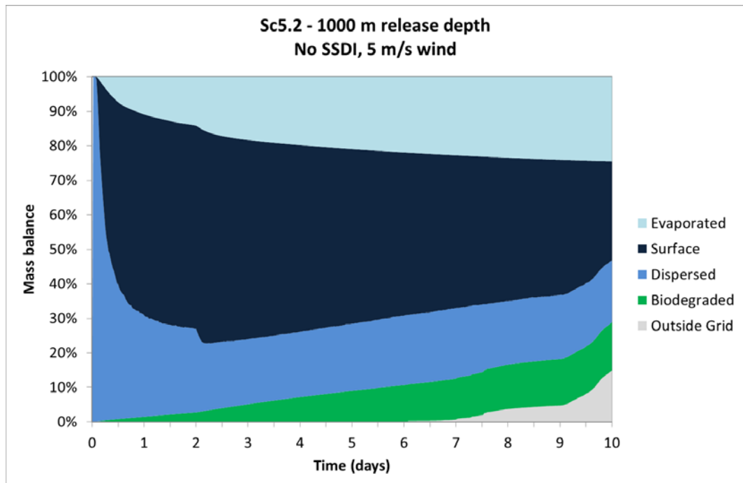
Figure A 5 Mass balance scenario 5.2
