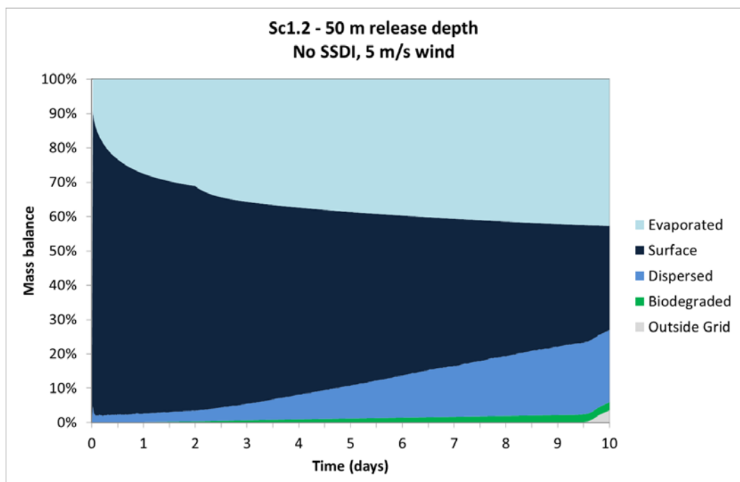
Figure A 2 Mass balance scenario 1.2
