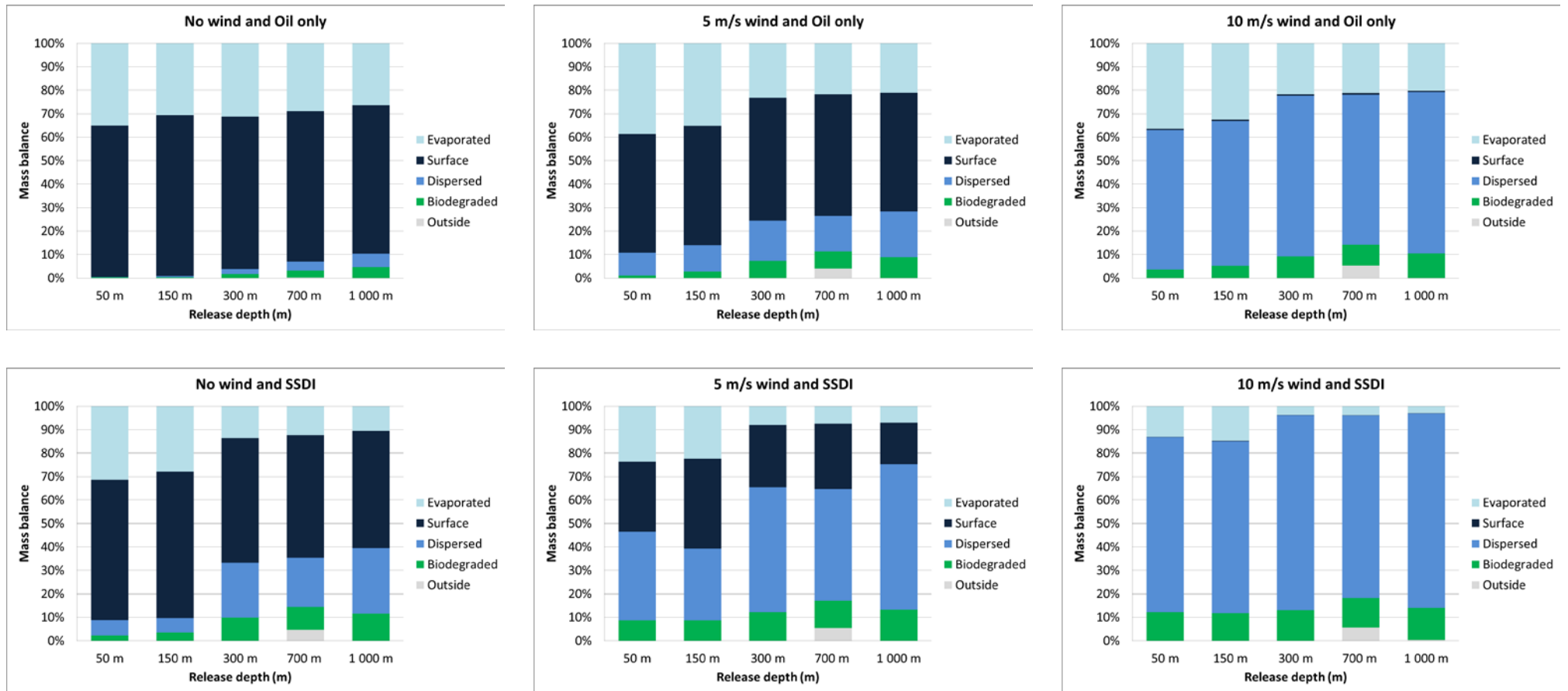
Figure 4.2 Mass balance 5 days into the simulation period (3 days after the end of the release) for all scenarios. The upper pictures show the results for the scenarios without SSDI, whereas the lower pictures are the scenarios with SSDI. Left: No wind. Middle: 5 m/s wind. Right: 10 m/s wind.
