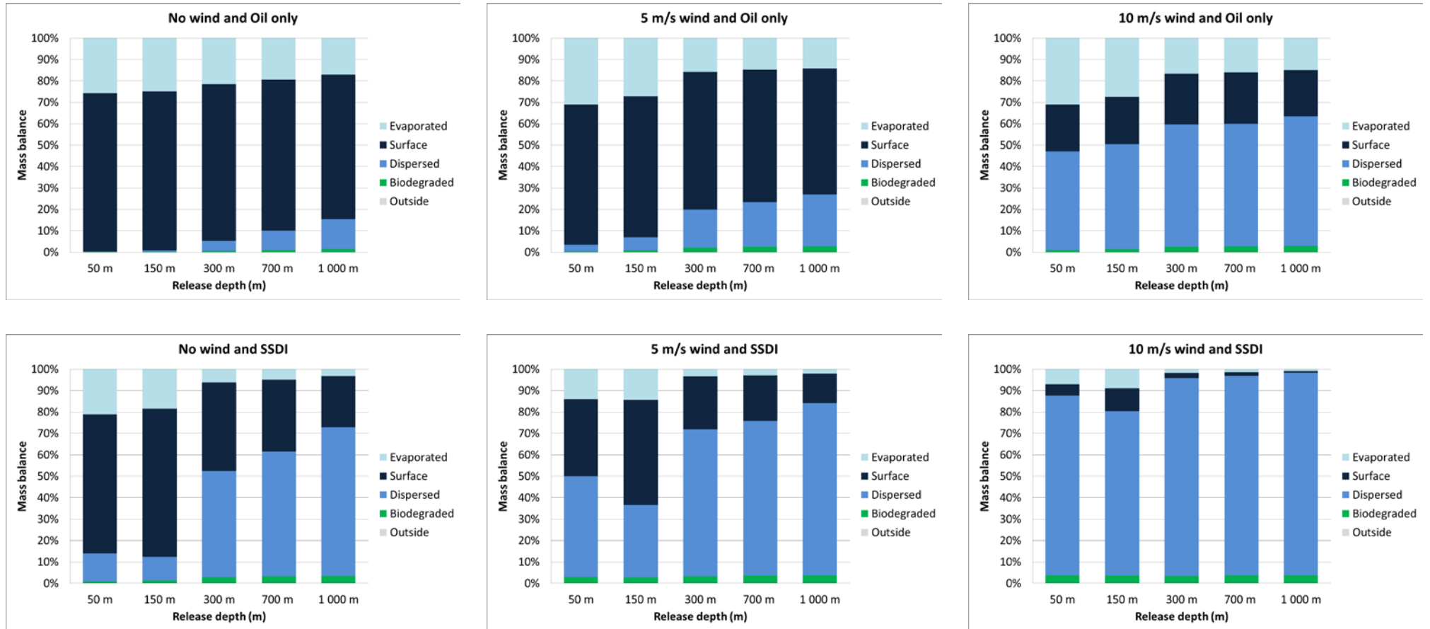
Figure 4.1 Mass balance 2 days into the simulation period (at the end of the release) for all scenarios. The upper pictures show the results for the scenarios without SSDI, whereas the lower pictures are the scenarios with SSDI. Left: No wind. Middle: 5 m/s wind. Right: 10 m/s wind.
