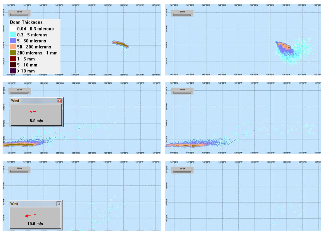
Figure 4.20 Surface oil at the end of the simulation period (10 days) for releases at 700 m depth. Left – oil only: No wind (upper), 5 m/s wind (middle) and 10 m/s wind (lower). Right – with SSDI: No wind (upper), 5 m/s wind (middle) and 10 m/s wind (lower).
