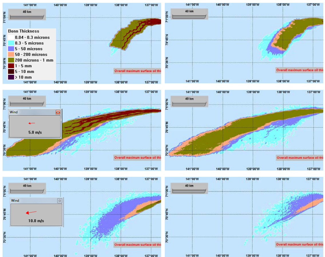
Figure 4.17 Overall maximum surface oil thickness (impacted area) for all releases at 300 m. Left – oil only: No wind (upper), 5 m/s wind (middle) and 10 m/s wind (lower). Right – with SSDI: No wind (upper), 5 m/s wind (middle) and 10 m/s wind (lower).
