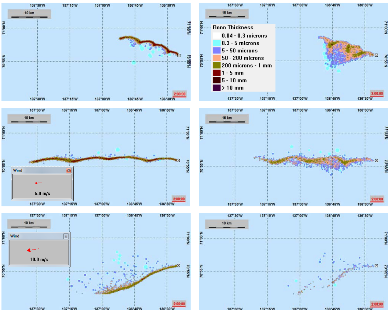
Figure 5.5 Surface oil at the end of the release for releases at 700 m depth. Left – no SSDI: No wind (upper), 5 m/s wind (middle) and 10 m/s wind (lower). Right – with SSDI: No wind (upper), 5 m/s wind (middle) and 10 m/s wind (lower).
