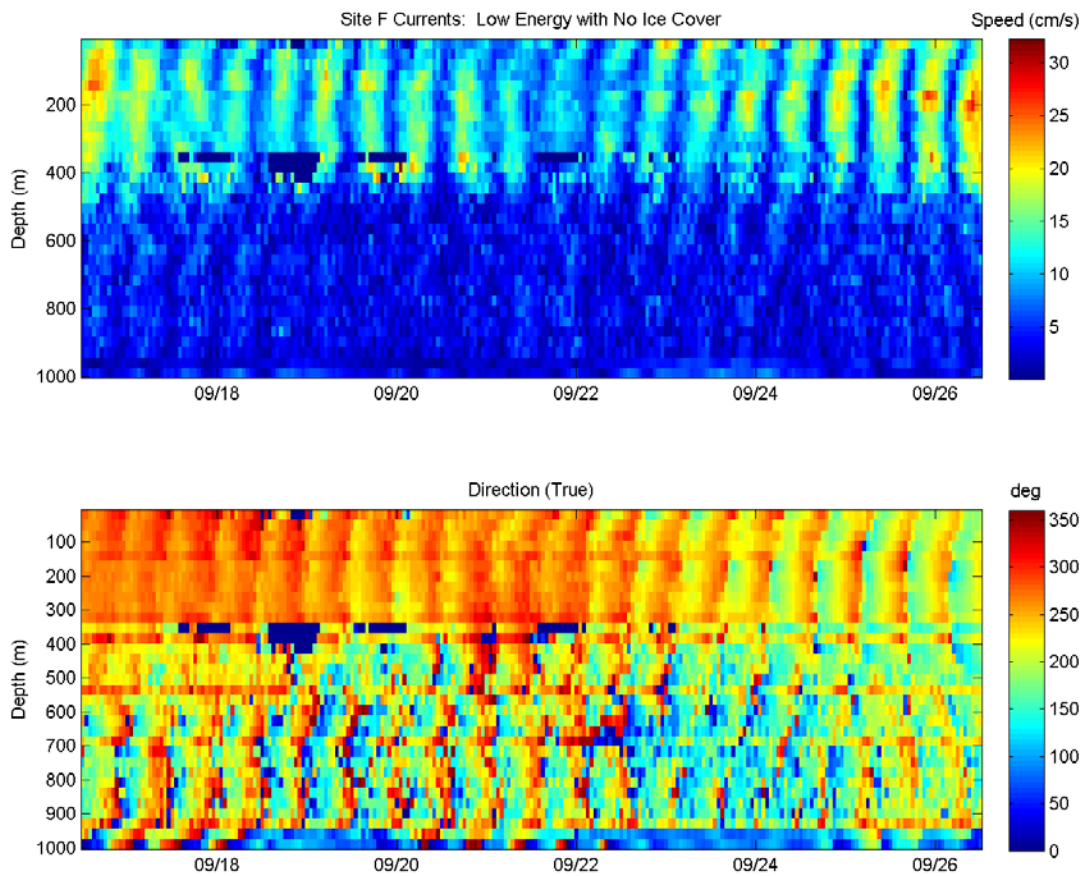
Figure 3.4 Current profile time series with weak/normal current conditions (from ASL, 2013).
