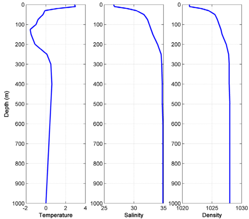
Figure 3.5 Temperature, salinity and density profiles used in the model scenarios.
