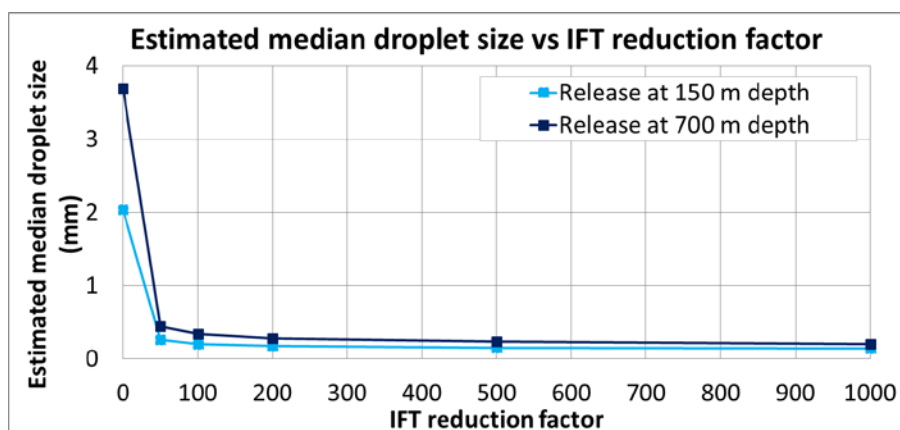
Figure 3.1 Estimated median droplet size for release depths at 150 and 700 m depth versus different interfacial tension (IFT) reduction factors. For this study, a reduction factor of 100 was chosen.
