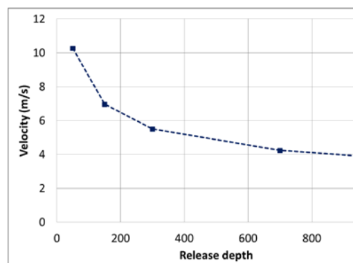
Figure 5.3 Buoyancy corrected release velocity for the different release depths.
