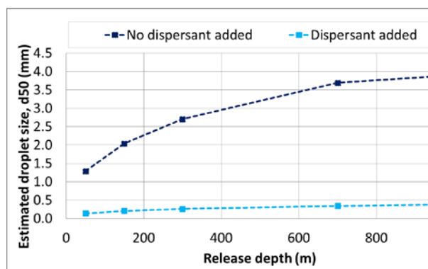
Figure 5.2 Estimated median droplet size for the different release depths with and without subsea injection of dispersants.
