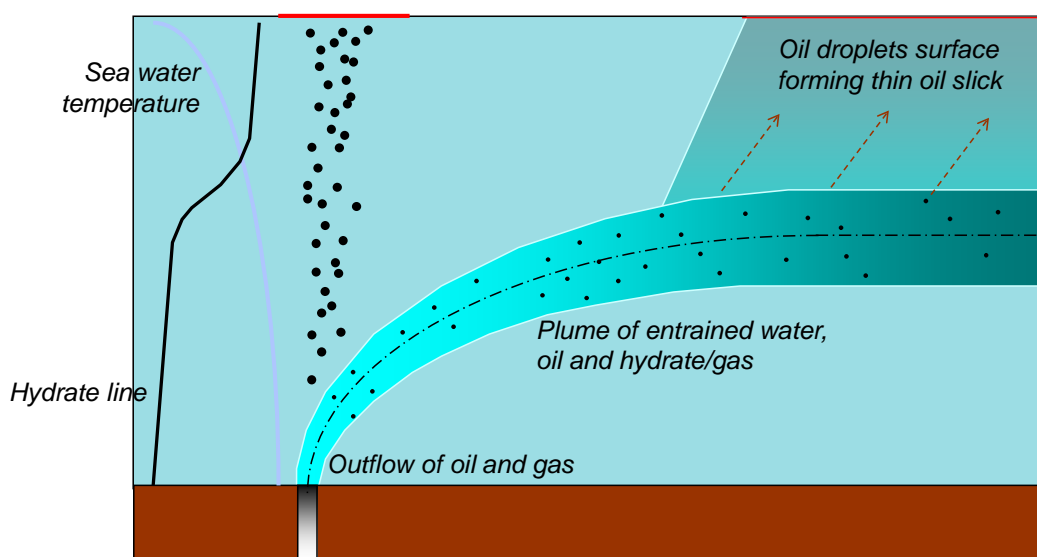
Figure 2.1 Diagram of a modelled plume. The oil and gas forms a buoyancy driven plume which may be trapped at a depth, as in this figure. Oil droplets escape the plume and are transported to the surface as a function of their size and corresponding buoyancy.
