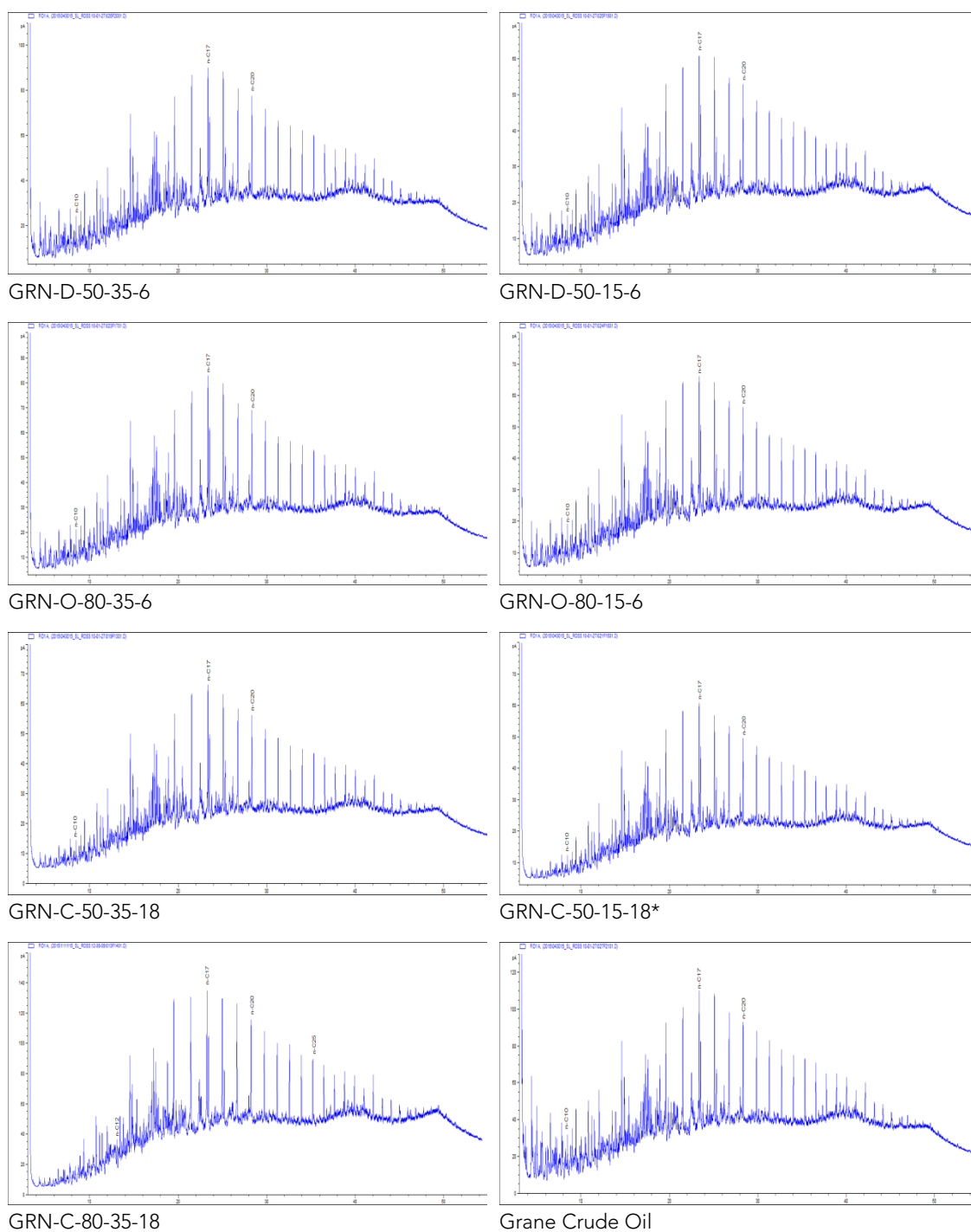
Figure D 5 GC chromatograms of Grane crude oil weathered in the flume prior to dispersant testing. Explanation of test identifications is provided in Table 2.6.
