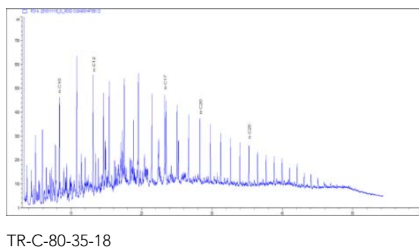
Figure D 4 GC chromatograms of Troll crude oil weathered for 18 hrs in the flume prior to dispersant testing. Explanation of test identifications is provided in Table 2.6.
