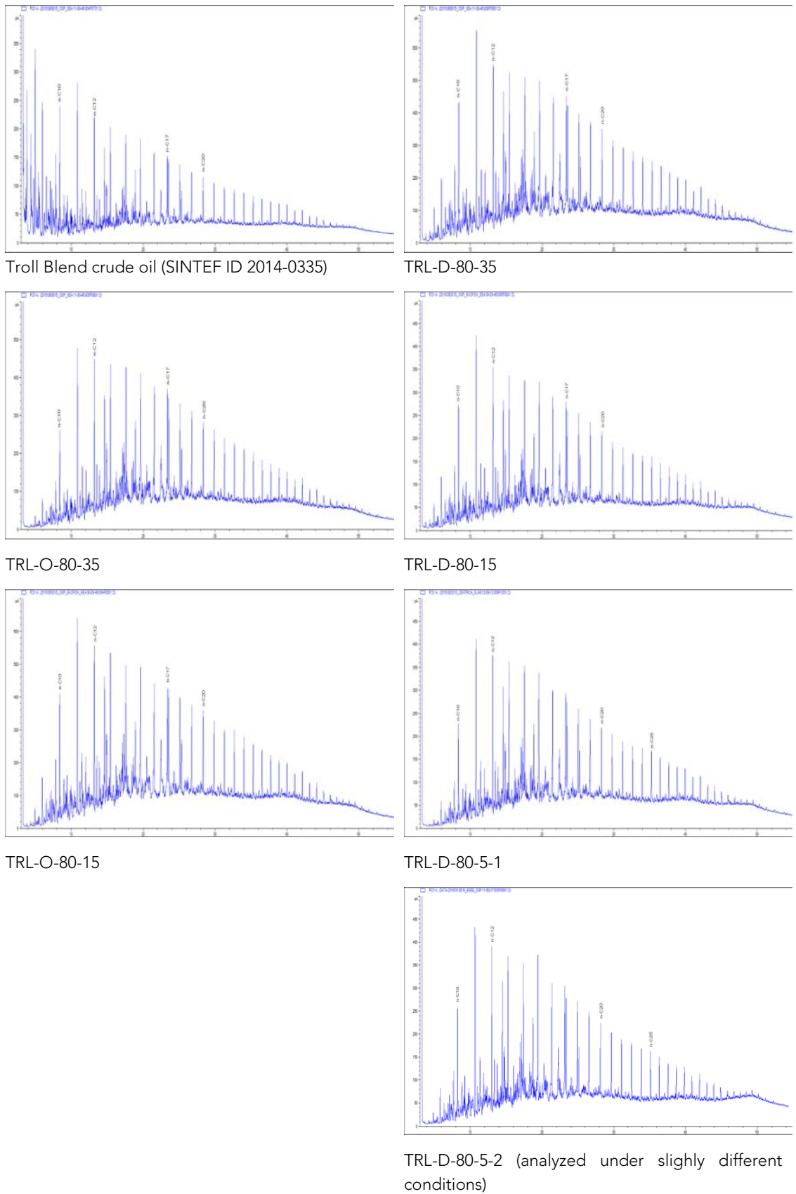
Figure C.2 GC chromatograms of Troll Blend weathered for 18 hrs in the flume prior to dispersant testing. Explanation of test identifications is provided in Table 2.5.
