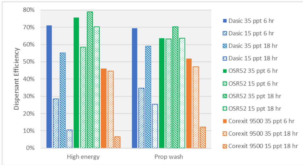
Figure B 1 Dispersant efficiency for Alaska North Slope crude oil
