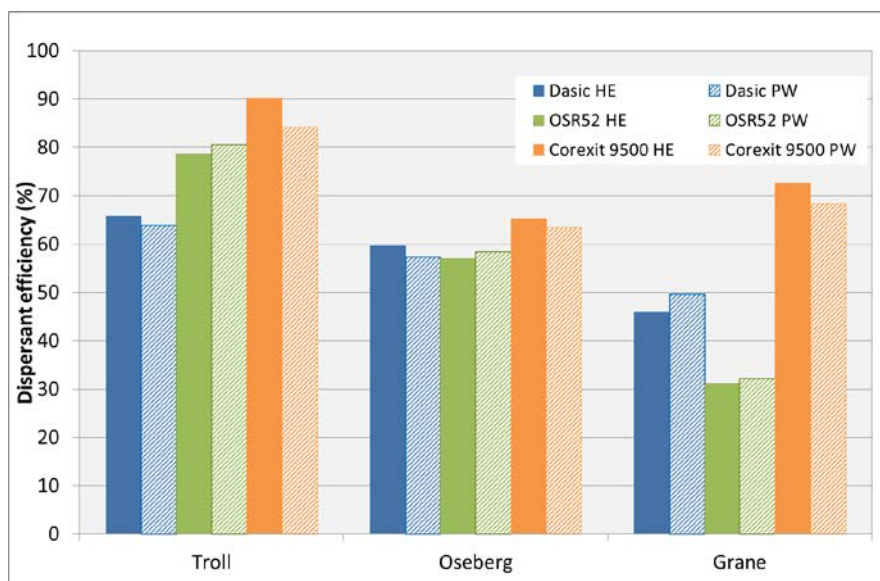
Figure A 4 Comparing dispersant efficiency in 35 ppt salinity water for the three oil types (HE: High energy, PW: prop wash).
