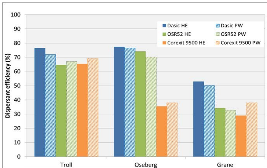
Figure A 5 Comparing dispersant efficiency in 15 ppt salinity water for the three oil types (HE: High energy, PW: prop wash).
