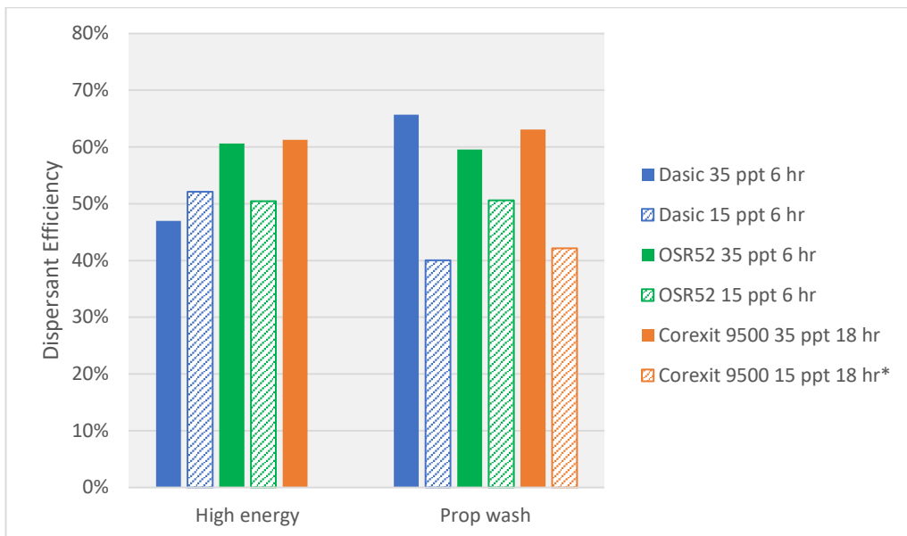
Figure B 2 Dispersant efficiency for Grane crude oil
