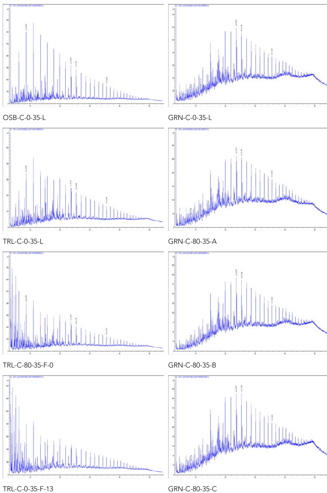
Figure C 4 GC chromatograms of the oils prior to dispersant application. Explanation of test identifications is provided in Table 4.1.
