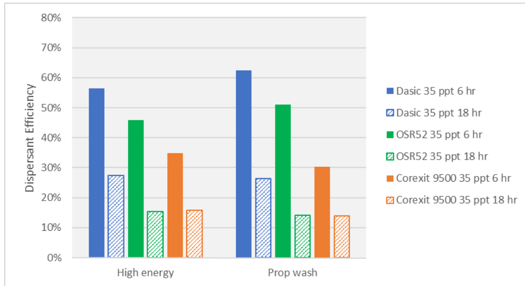
Figure B 3 Dispersant efficiency for IFO 80
