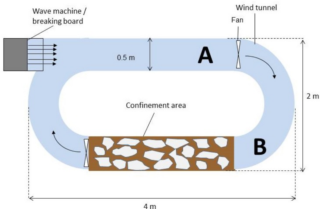
Figure 2.1 Sketch of the SINTEF and SL Ross flume
