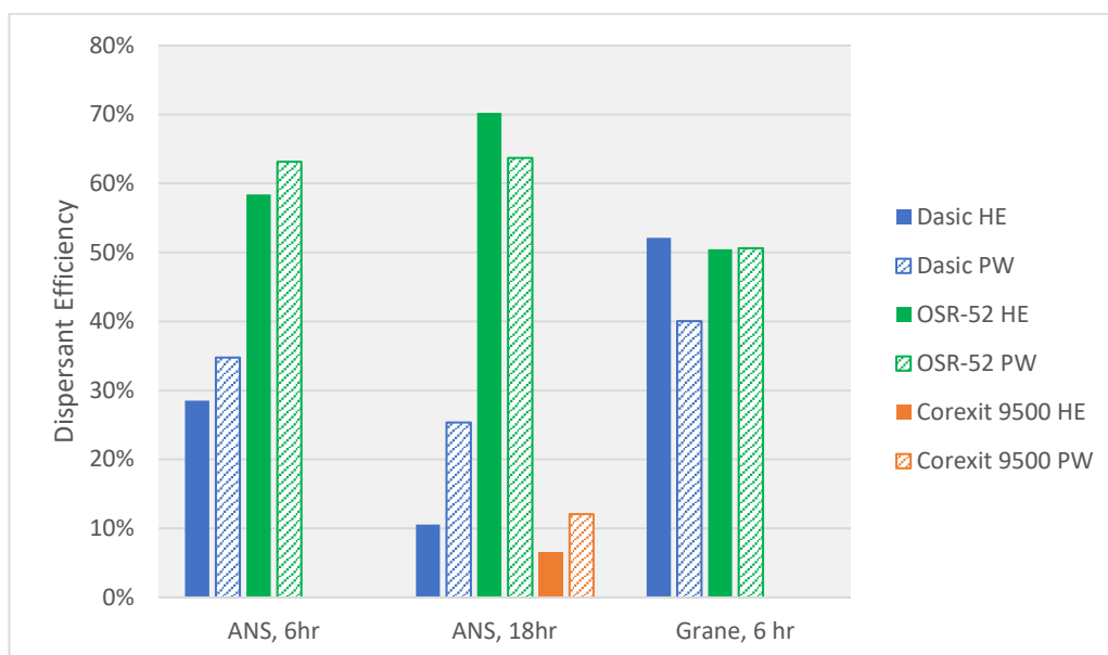
Figure B 5 Dispersant efficiency in 15 ppt salinity water for ANS and Grane crude oils (HE: High energy, PW: prop wash).
