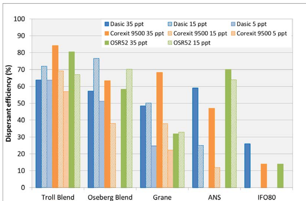
Figure 3.3 Dispersant efficiency vs water salinity. Oils were weathered for 18 hrs in 80% ice. DE measured from water grab samples collected after prop wash. No bars indicate that no testing was performed.
