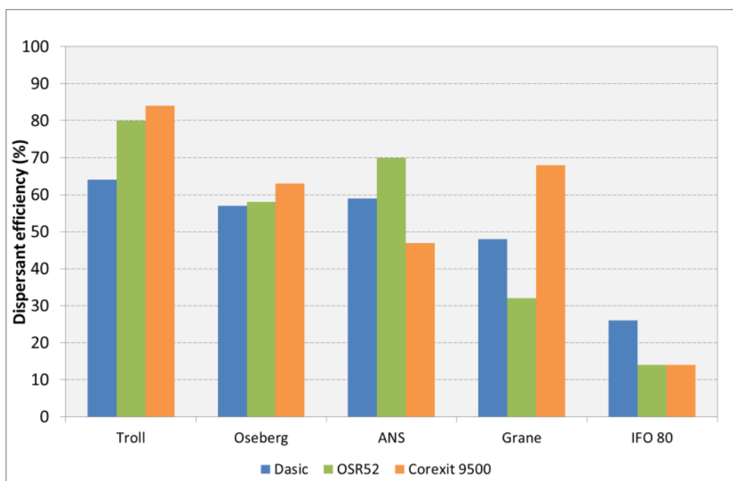
Figure 3.1 Dispersant efficiency vs dispersant type. Oils were weathered for 18 hrs in 80% ice and 35 ppt salinity water. DE measured from water grab samples collected after prop wash.
