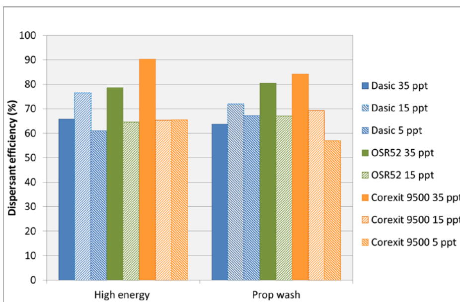
Figure A 1 Dispersant efficiency for Troll Blend
