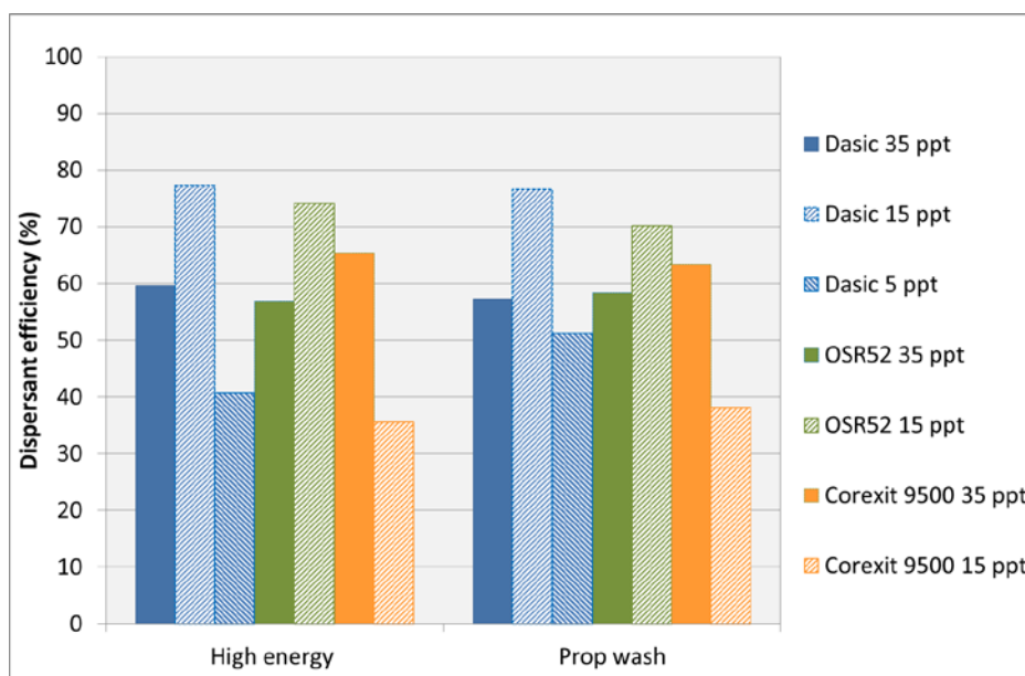
Figure A 2 Dispersant efficiency for Oseberg Blend
