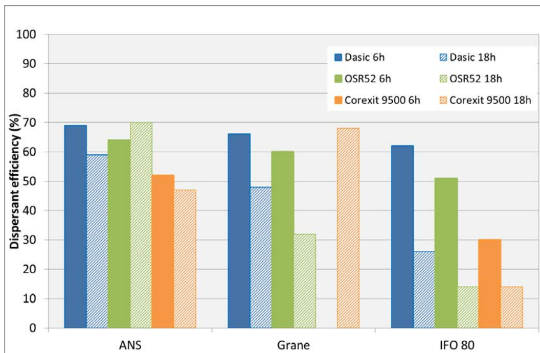
Figure 3.2 Dispersant efficiency vs weathering time. Oils were weathered for 6 hrs or 18 hrs in 80% ice and 35 ppt salinity water (Grane Corexit 9500 6hrs not performed). DE measured from water grab samples collected after prop wash
