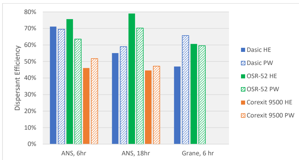
Figure B 4 Dispersant efficiency in 35 ppt salinity water for ANS and Grane crude oils (HE: High energy, PW: prop wash).
