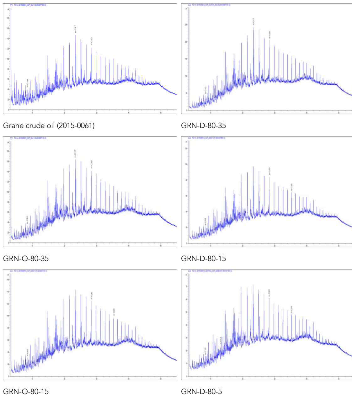
Figure C 3 GC chromatograms of Grane crude oil weathered for 18 hrs in the flume prior to dispersant testing. Explanation of test identifications is provided in Table 2.5.
