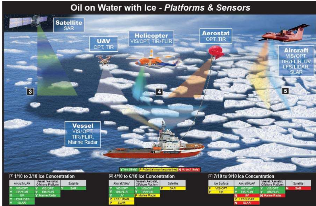
Figure 3-3 Platforms and Sensors for Oil on Water with Varying Ice Concentrations (Categories 3 – 5)
