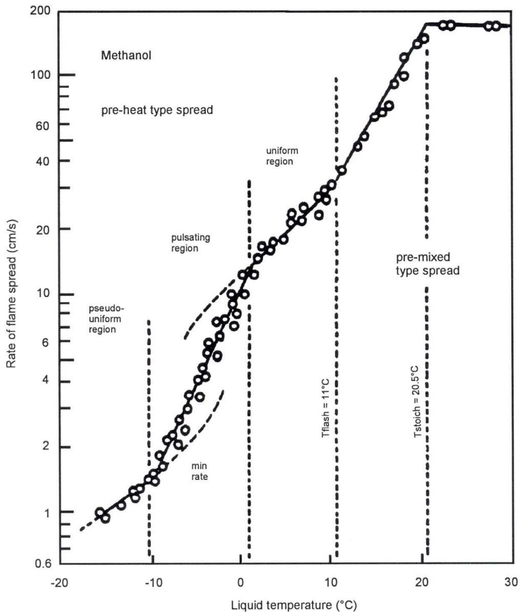
Figure 4-10 Relationship between the liquid temperature and the rate of plane flame spread of methanol in a vessel 2.6-cm wide and 1.0-cm deep. (Source: Marine Spill Response Corporation)
