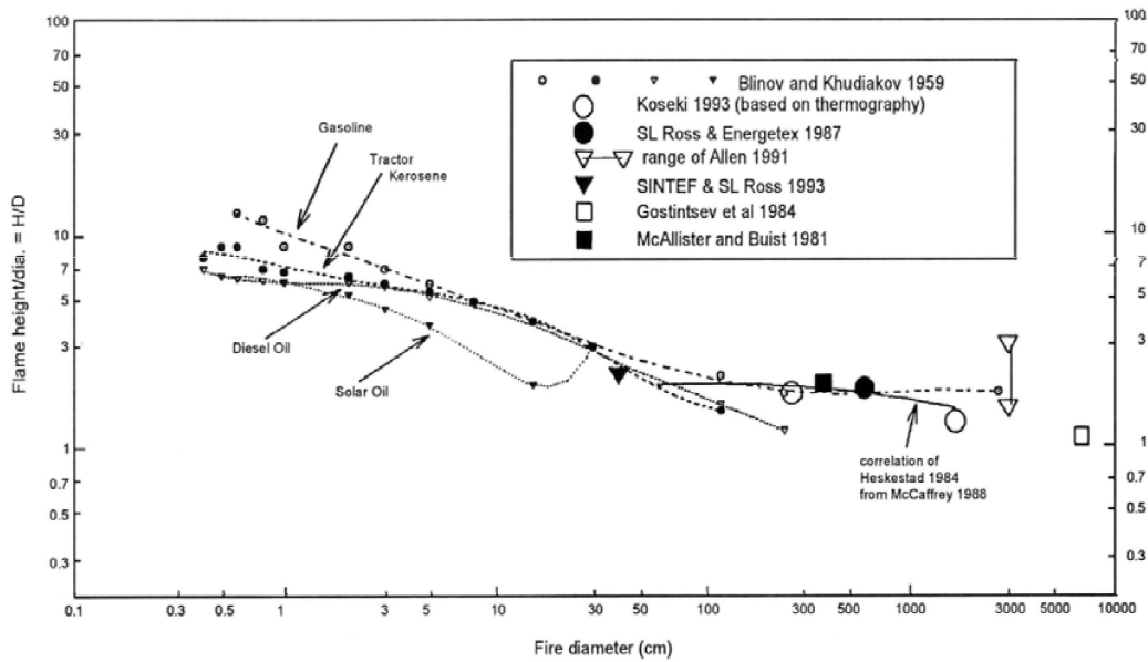
Figure 4-14 Flame height vs. fire diameter - a comparison of data sets. (Source: Marine Spill Response Corporation)
