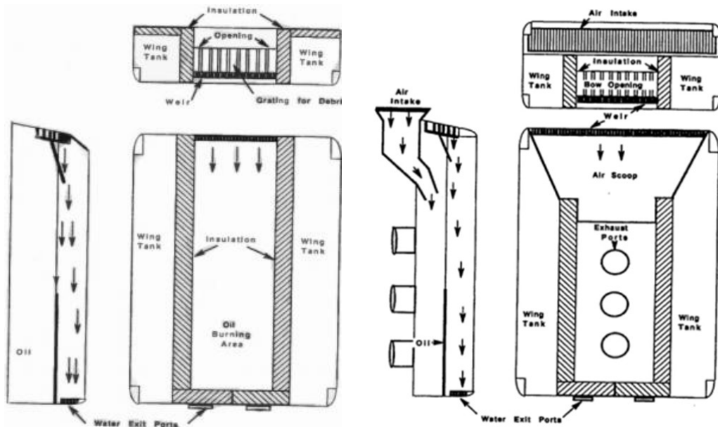
Figure 6-24 Simple, modified existing barge hull concept. (Source: Marine Research Associates)
