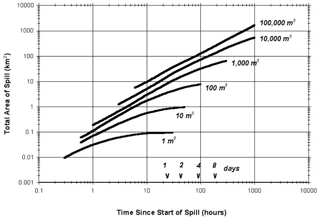
Figure 3-4 Predicted Spreading of Spills on Open Water. (Source: SL Ross Environmental Research)
