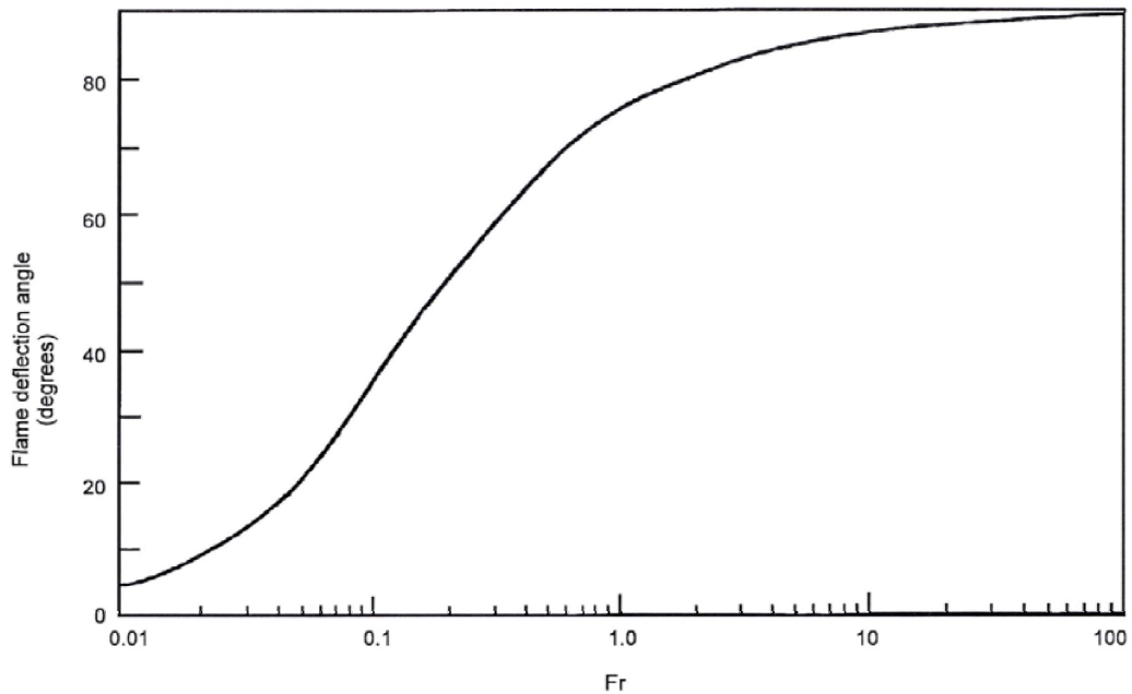
Figure 4-15 Flame deflection angle as a function of the kinematic Froude number, from Eq. 4-13 (from Brzustowski & Twardus, 1982). (Source: Marine Spill Response Corporation)
