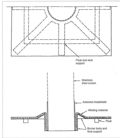
Wicking burner. (From Twardus, 1978)
