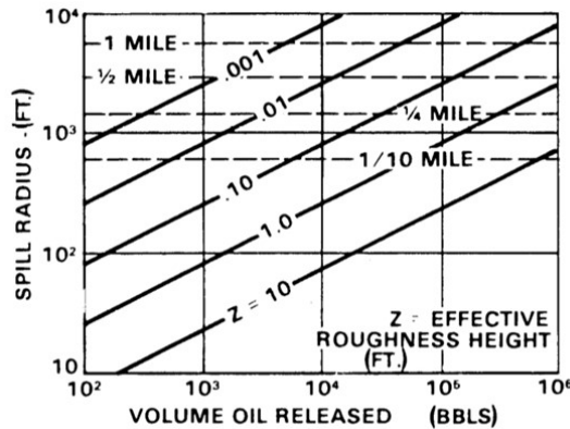
Figure 3-2 Predicted Spreading of Spilled Oil on Ice (McMinn 1972) (source: SL Ross Environmental Research)
