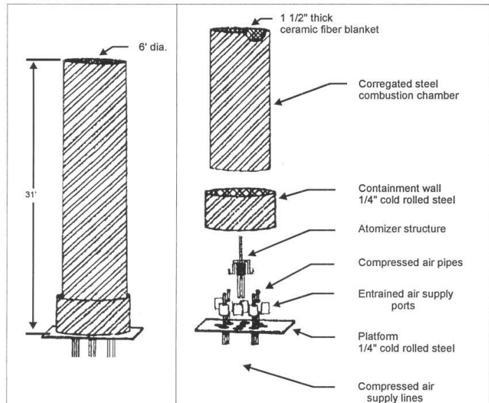
Figure 6-19 Two-metre diameter incinerator. (From Franken et al. , 1992)
