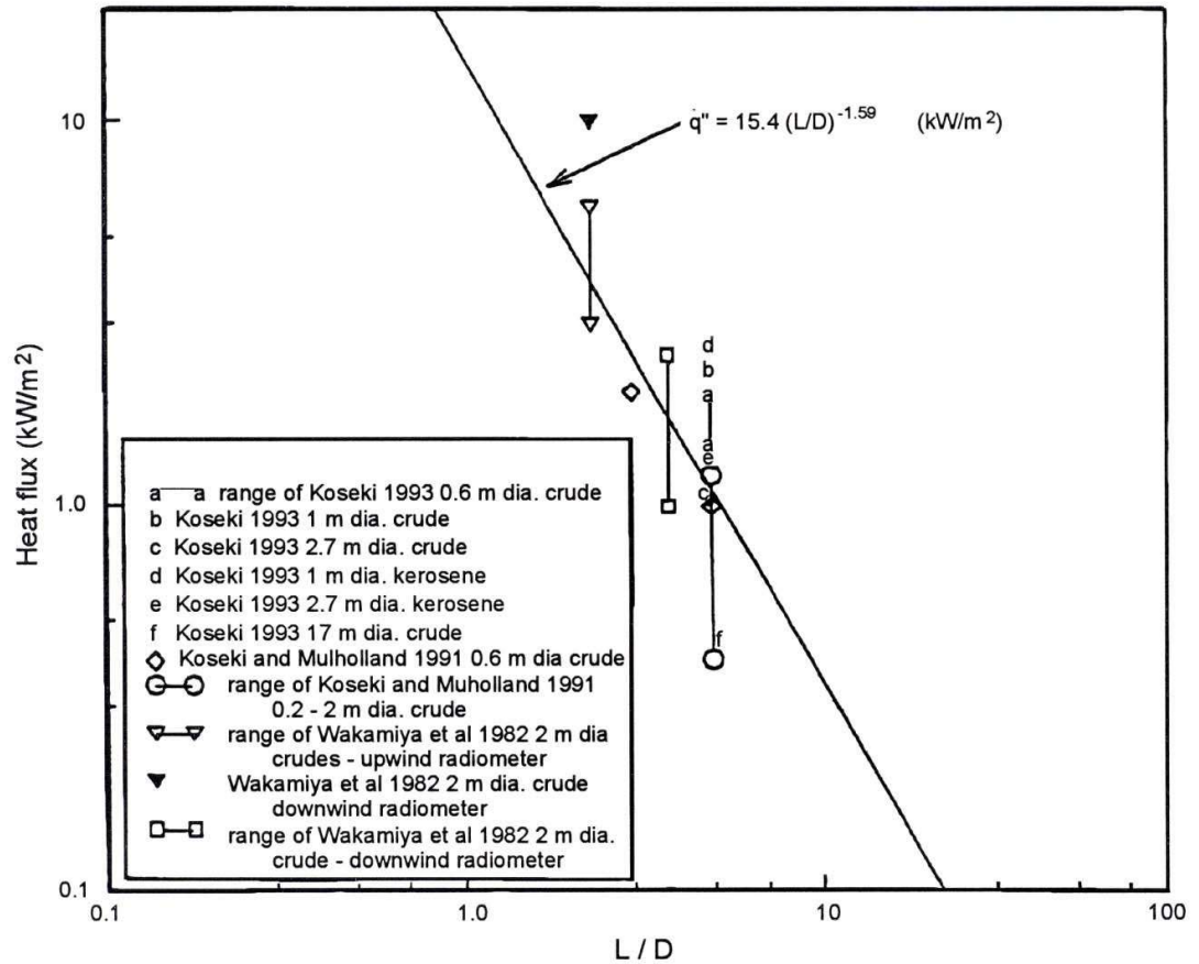
Figure 4-16 External heat flux from burning - comparison of Shokri & Beyler's (1989) correlation with in situ burn data. (Source: Marine Spill Response Corporation)
