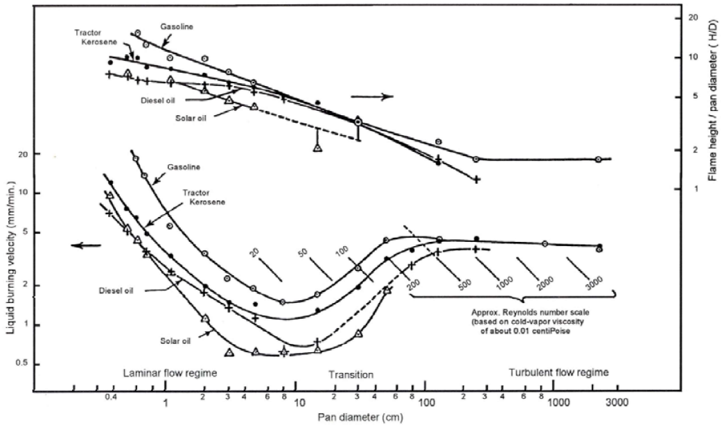
Figure 4-2 Burning data (from Blinov & Khudiakov 1959). (Source: Marine Spill Response Corporation)
