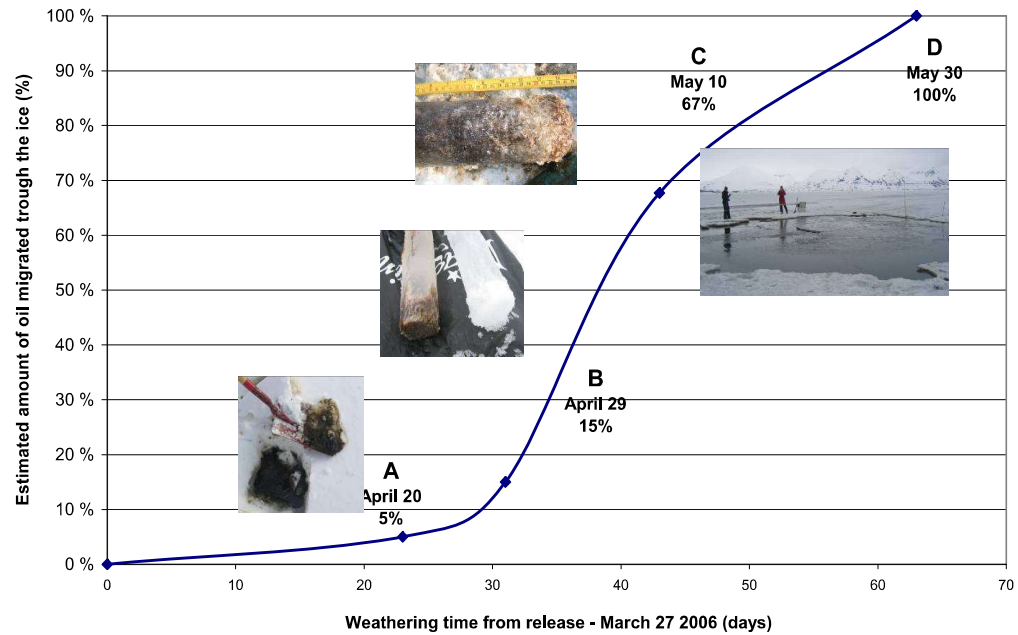
Figure 3-8 Estimated Amount of Oil Penetrated through the Brine Channels in the Ice and Available on the Ice Surface during SINTEF's Experimental Spill Under Ice in 2006 Photos show appearance of cores at different stages in the migration cycle. (Source: SINTEF/UNIS)
