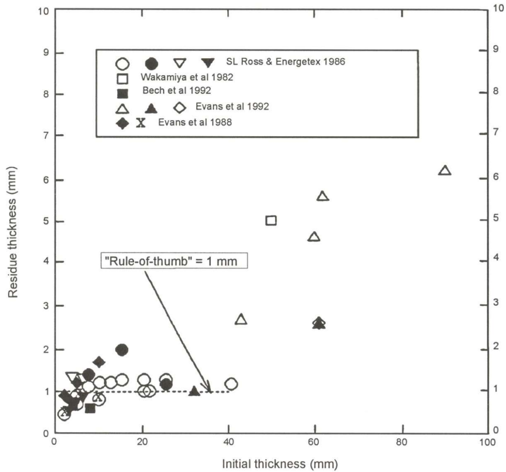
Figure 4-7 Residue thickness as a function of initial slick thickness. (Source: Marine Spill Response Corporation)
