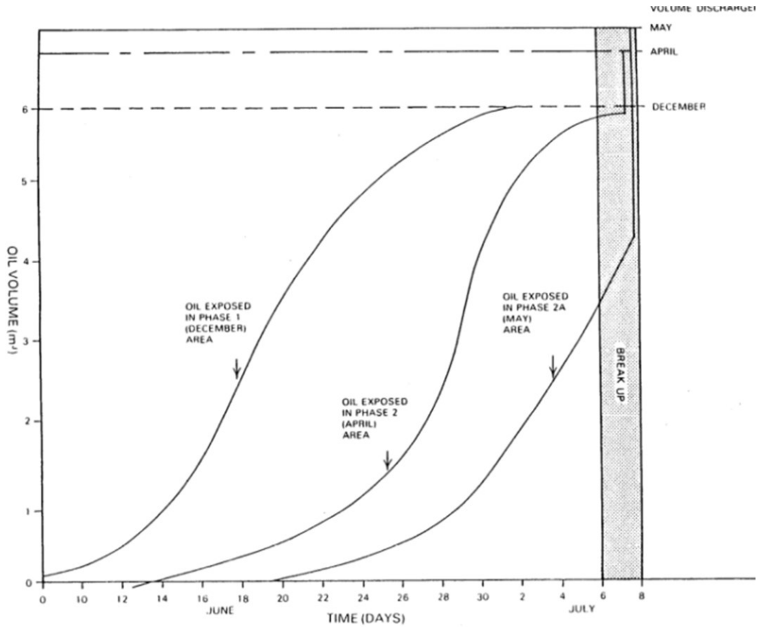
Figure 3-6 Initial Surface Appearance of Crude Oil Migrating Through the Ice at the Dome Oil and Gas Under Sea Ice Experiment in Early June 1980. (Source: D. Dickins)
