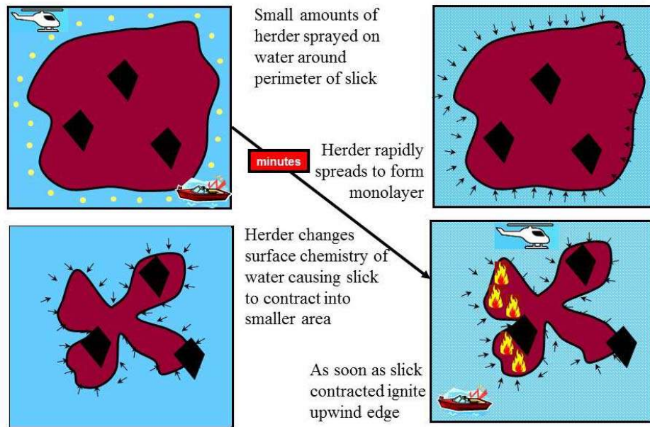
Figure 6-6 Concept for use of herders to contract oil slicks in drift ice for ignition and burning. (Source: SL Ross Environmental Research)
