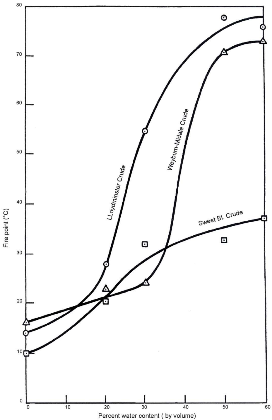
Figure 4-18 W/O emulsion fire points vs. water content (from Energetex 1980). (Source: Marine Spill Response Corporation)
