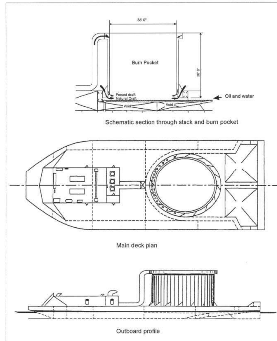
General arrangement of Arctic incinerator barge. (From Glosten et al. , 1991)
