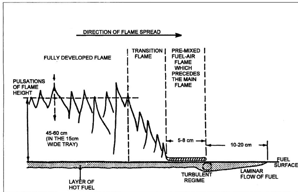
Figure 4-11 Schematic representation of the spreading flame. (Source: Marine Spill Response Corporation)
