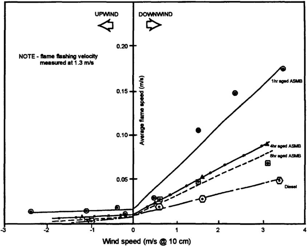
Figure 4-13 Flame spreading velocity. (Source: Marine Spill Response Corporation)
