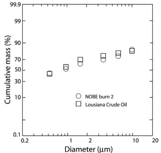
Figure 8-2 Particle size distributions in smoke plumes from large in situ burns. (From Evans et al. 2001)
