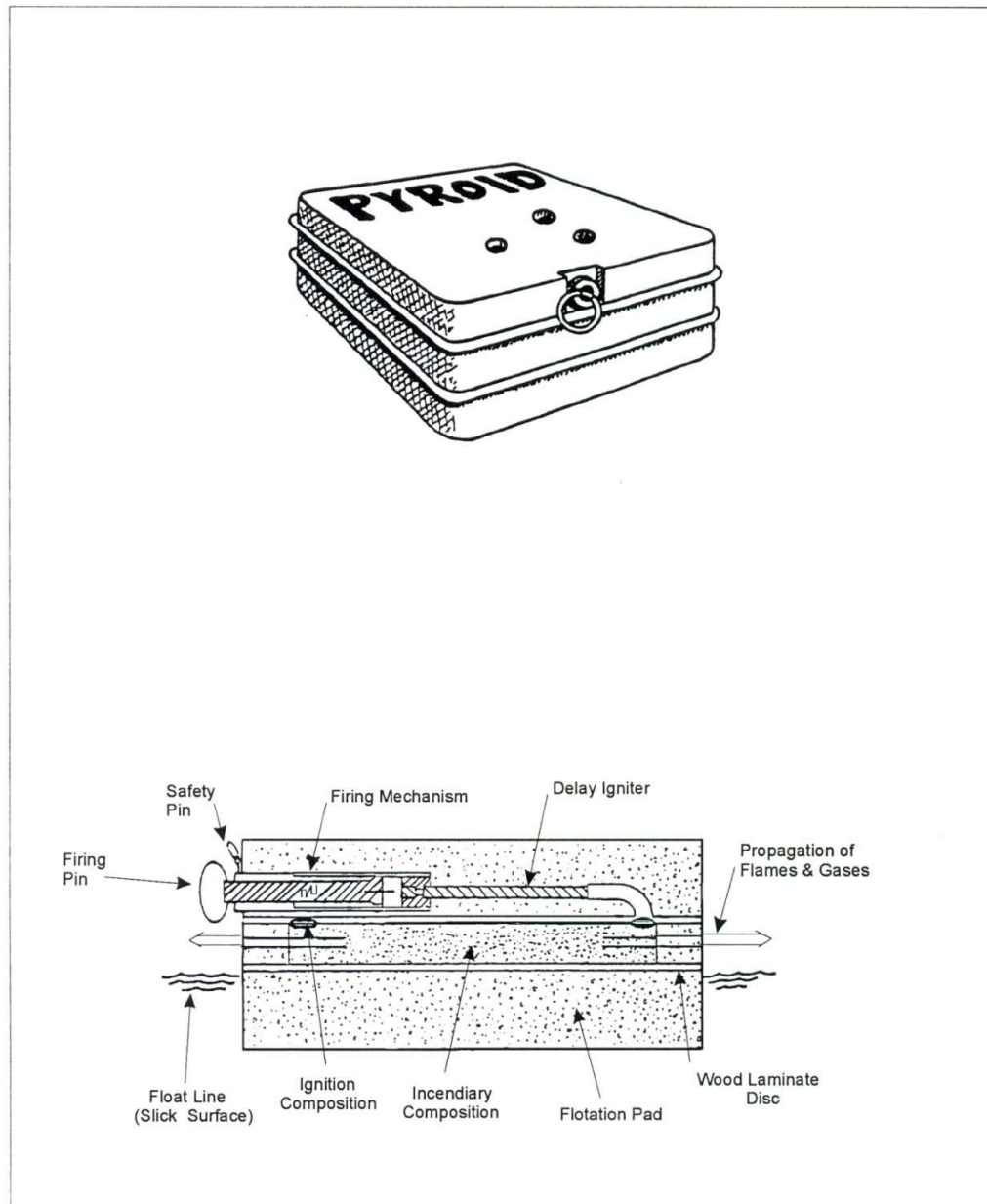
Figure 6-5 Environmental Protection Service (EPS) igniter, or Pyroid igniter, showing internal firing mechanism and pyrotechnic components (adapted from Allen 1986). (Source: Marine Spill Response Corporation)
