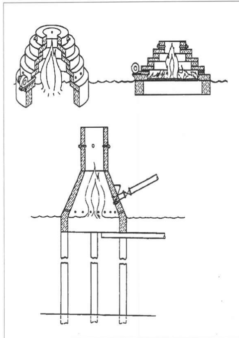
Floating oil spill furnace (from U.S. Patent 3,695,810 - October 3, 1972)
