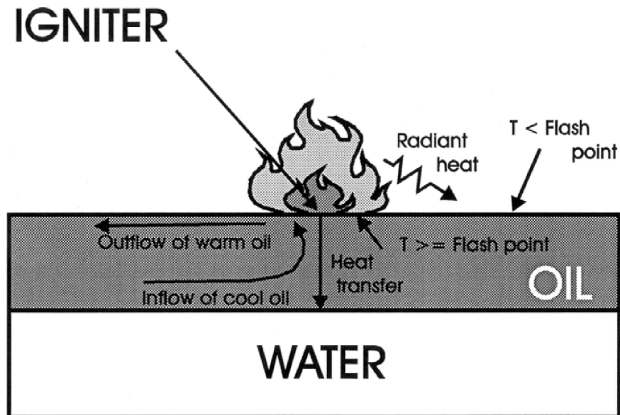
Figure 4-9 Heat transfer and convective motion during slick ignition. (Source: Marine Spill Response Corporation)
