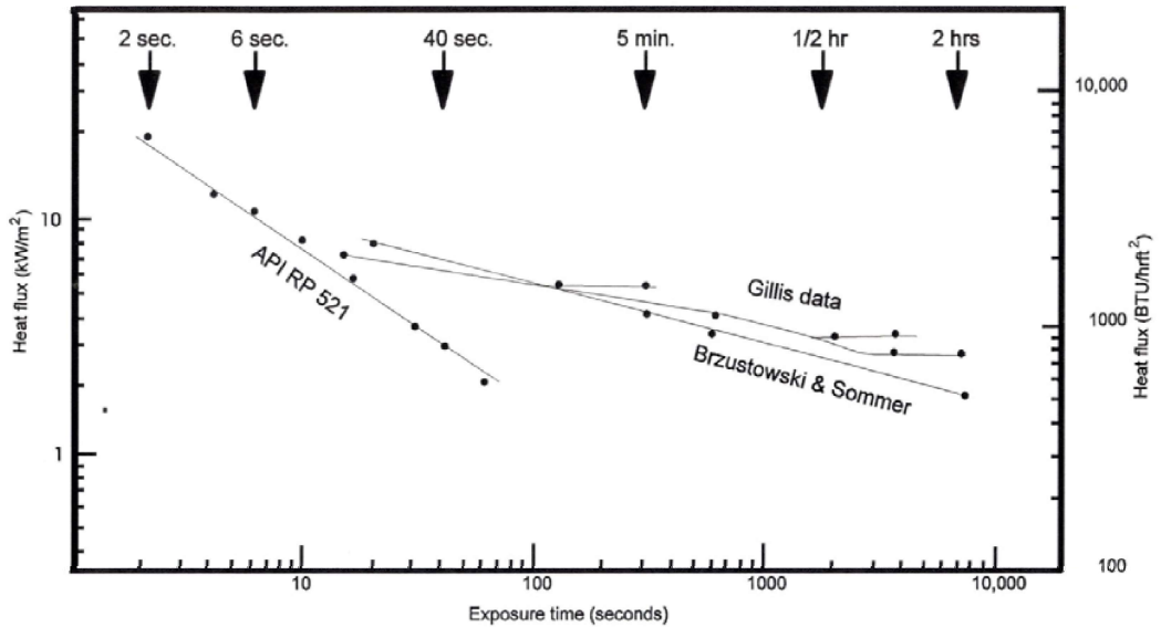
Figure 4-17 Allowable fluxes for personnel exposure (adapted from Oenbring & Sifferman, 1980). (Source: Marine Spill Response Corporation)
