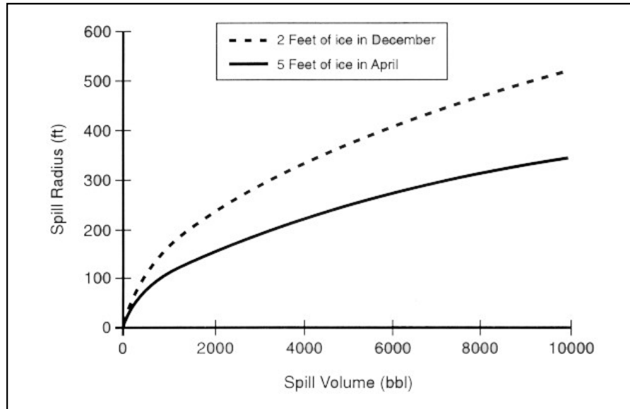
Figure 3-3 Predicted Radii of Spills of a Given Volume Spilled Under Landfast Ice (Dickins and Glover 1996. (Source: D. Dickins)
