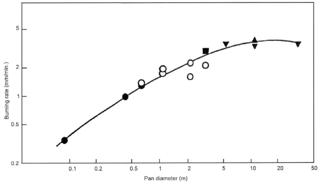
Figure 4-4 Relationship between burning rate and tank diameter (from Koseki & Mulholland, 1991). (Source: Marine Spill Response Corporation)
