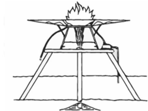
Figure 6-13 Combustion system for pipeline leaks (Source: U.S. Patent 3,602,299 - August 31, 1971)
