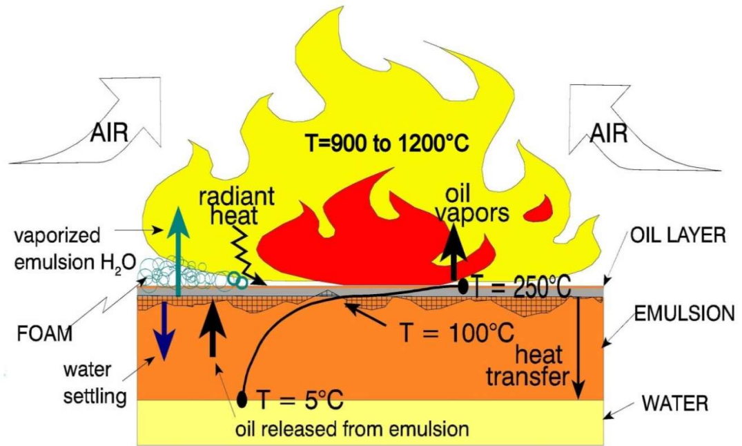
Figure 4-19 Key heat and mass transfer processes for in situ burning of emulsions. (Source: SL Ross Environmental Research)
