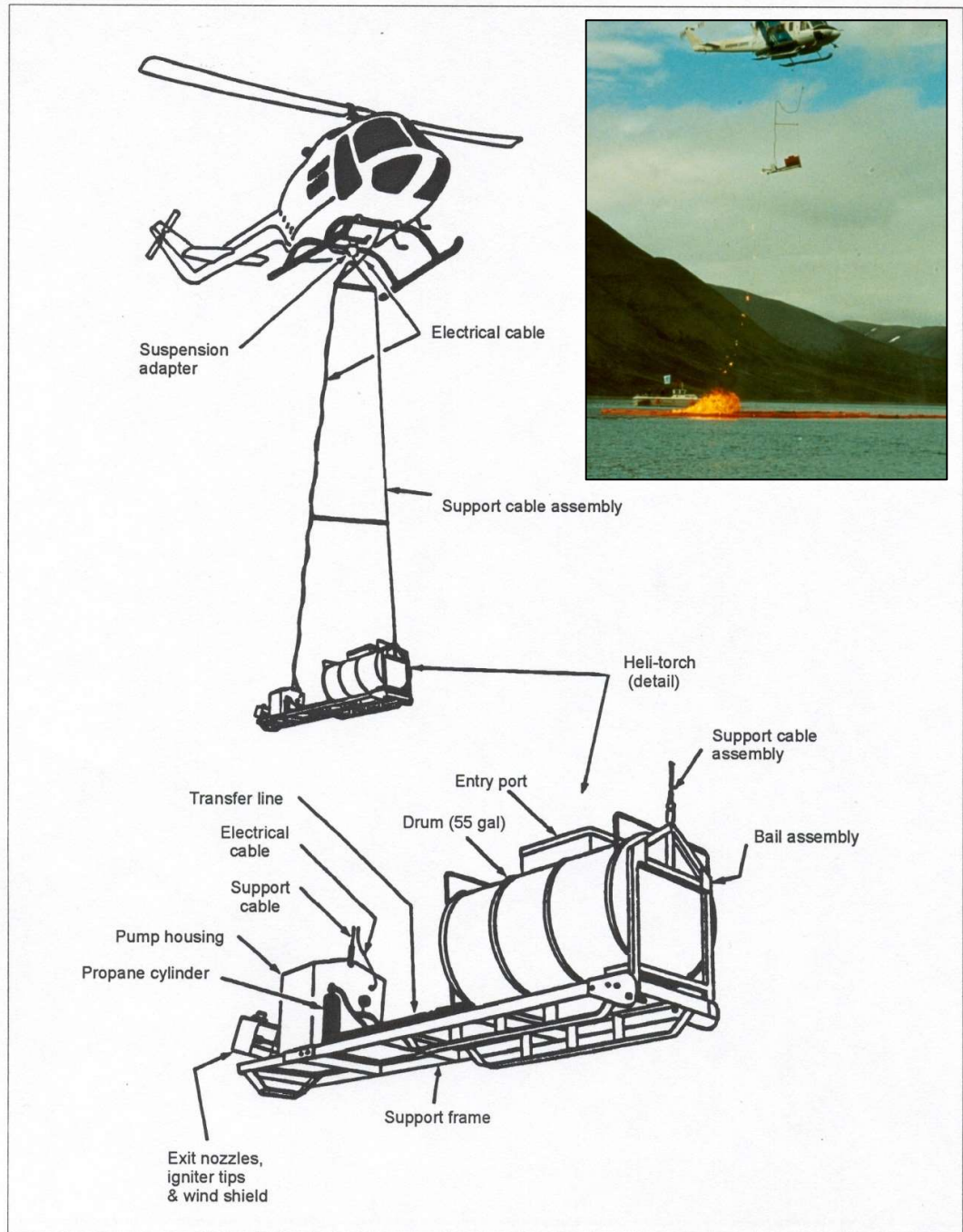
Figure 6-4 Heli-Torch Components and Support System (adapted from Allen 1986). (Source: Marine Spill Response Corporation; photo: A. Allen)
