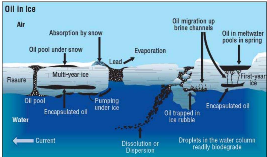
Figure 3-1 Illustration of Oil and Ice Processes (adapted from Borbra and Fingas 1981) (Source: ExxonMobil).
