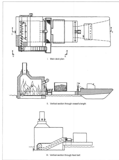
Oil spill incinerator vessel (from U.S. Patent 3,663,146 - May 16, 1972)
