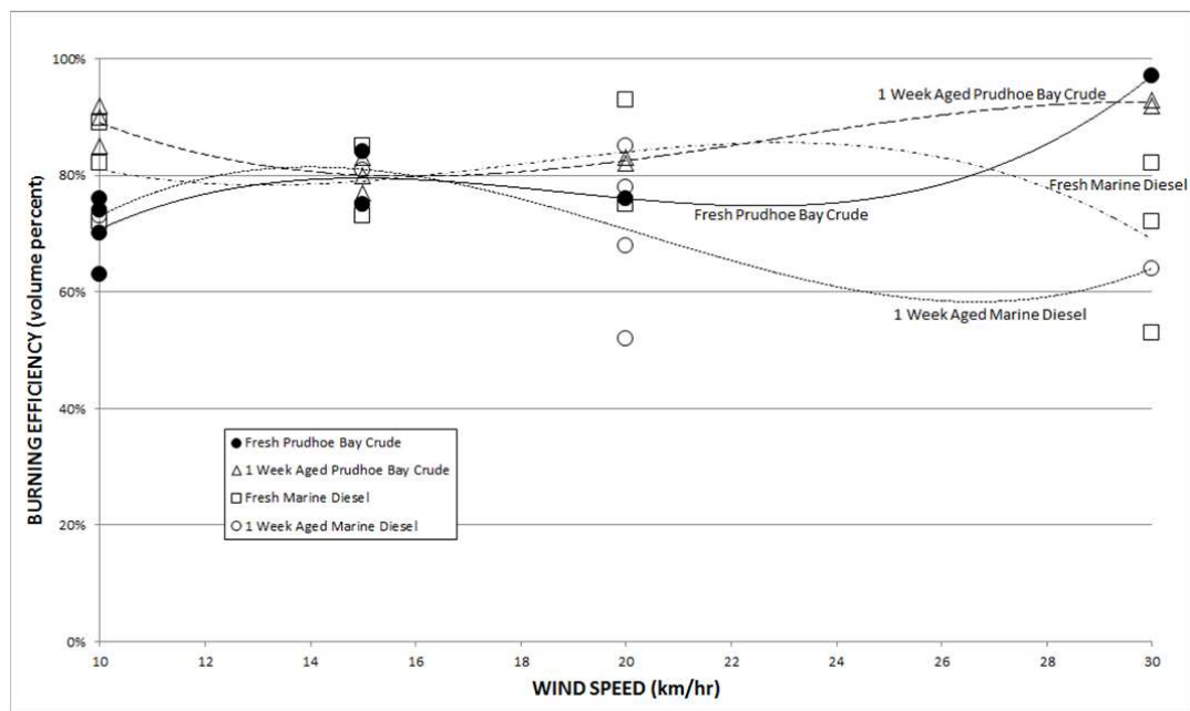
Figure 4-8 Removal efficiency vs. wind speed for 1m 2 burns (from Energetex 1981a). (Source: Marine Spill Response Corporation)
