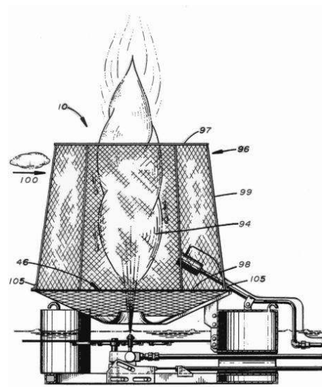
Sprayburn floating oil burner. (From U.S. Patent 5,057,004 - October 15, 1991)
