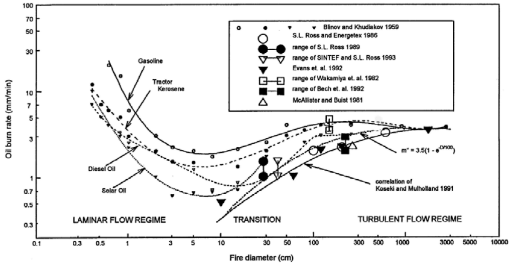
Figure 4-3 Burning rate vs. fire diameter - a comparison of data sets. (Source: Marine Spill Response Corporation)
