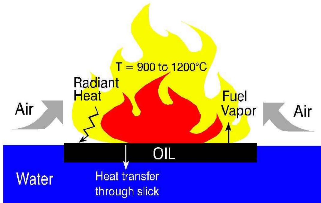
Figure 4-1 Key heat and mass transfer processes for in situ burning. (Source: SL Ross Environmental Research)
