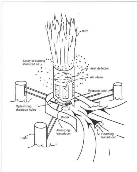
Figure 6-16 Combination of oil herding and atomizing device. (Source: MSRC)
