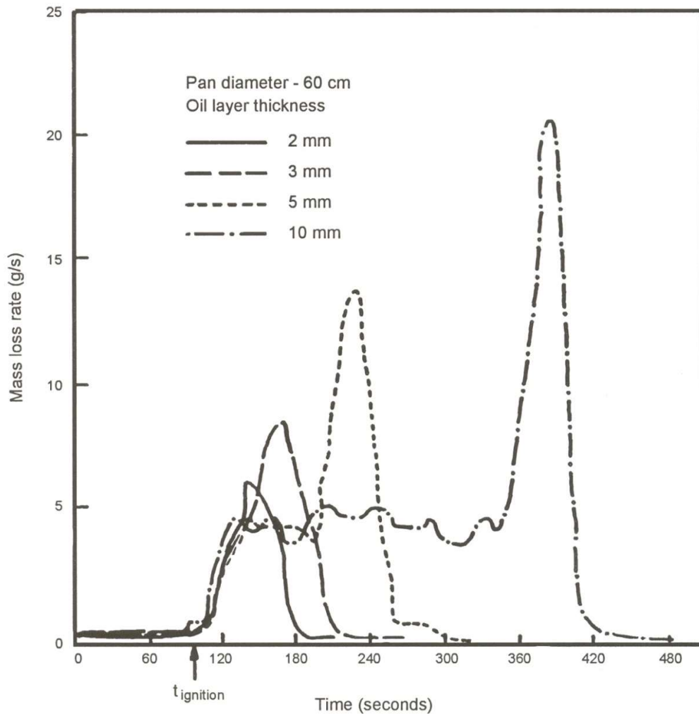
Figure 4-6 Effect of oil layer thickness on mass loss rate (fuel) for crude oil fires (from Evans et al. , 1988). (Source: Marine Spill Response Corporation)
