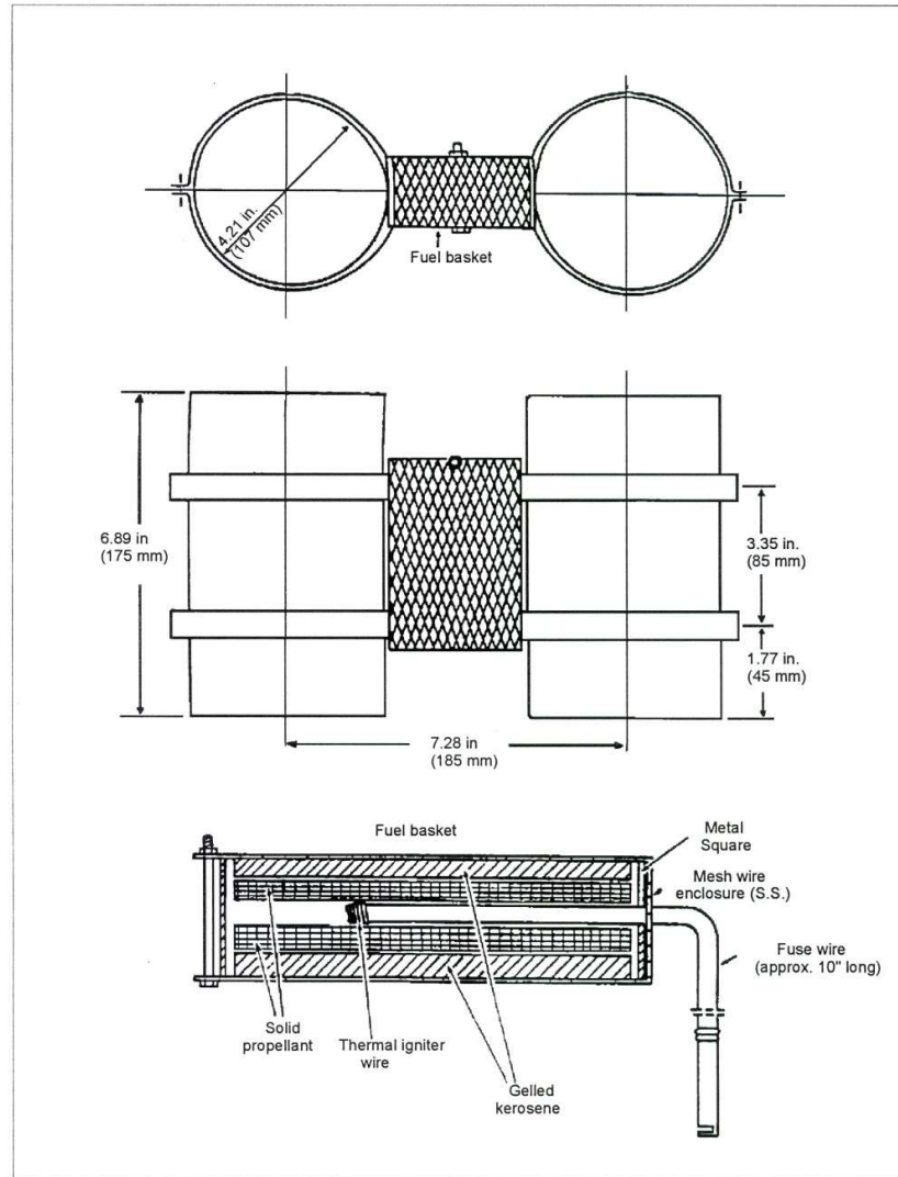
Figure 6-3 Basic design and internal components of the Dome or Energetex igniter (adapted from Allen, 1986). (Source: Marine Spill Response Corporation)
