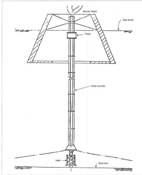
Figure 6-14 Dome subsea blowout burner. (From Buist & Potter, 1982)
