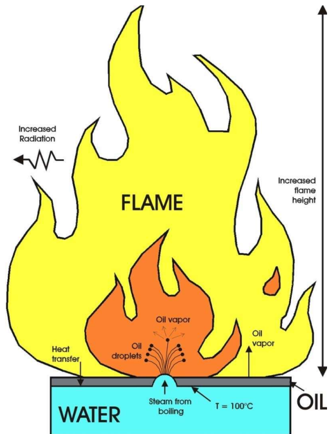
Figure 4-5 Development of the vigorous burning phase. (Source: Marine Spill Response Corporation)
