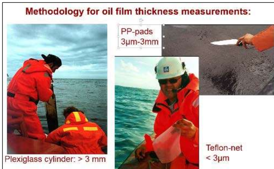
Figure 6.3 Methodologies for measuring oil slick thicknesses
