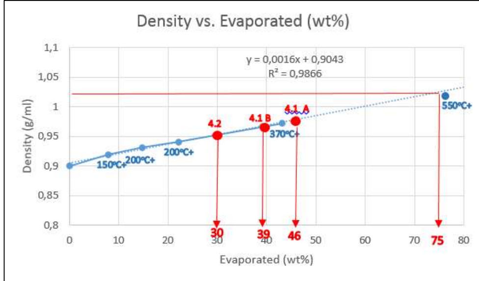
Figure E.2 Correlation (linear regression) between the densities and evaporative loss by topping of the Grane crude.
