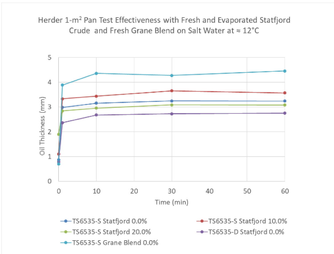
Figure 4.1 Bench Scale Herder Effectiveness Testing
