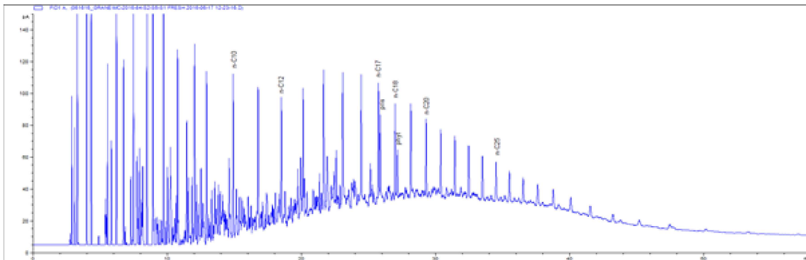
Figure 4.2 GC/FID chromatograms for the fresh oil samples of Grane Blend (2016).
