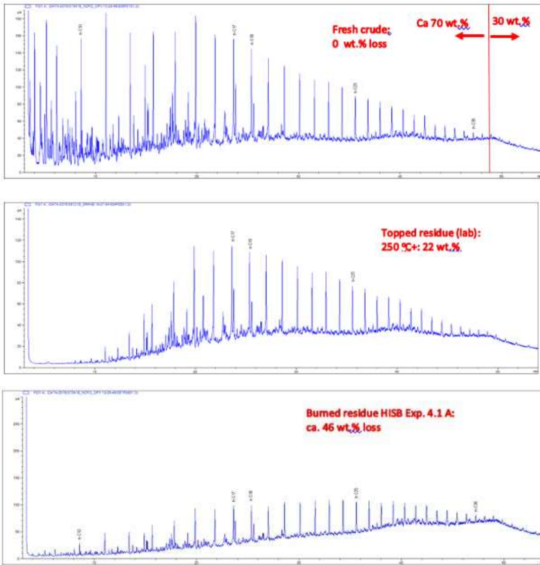
Figure E.1 GC-chromatograms of Grane Blend A: Fresh crude, B: laboratory topped residue at 250°C+, giving a quantified evaporative loss of 22 wt%., C: Burned residue (sample 4.1.A)
